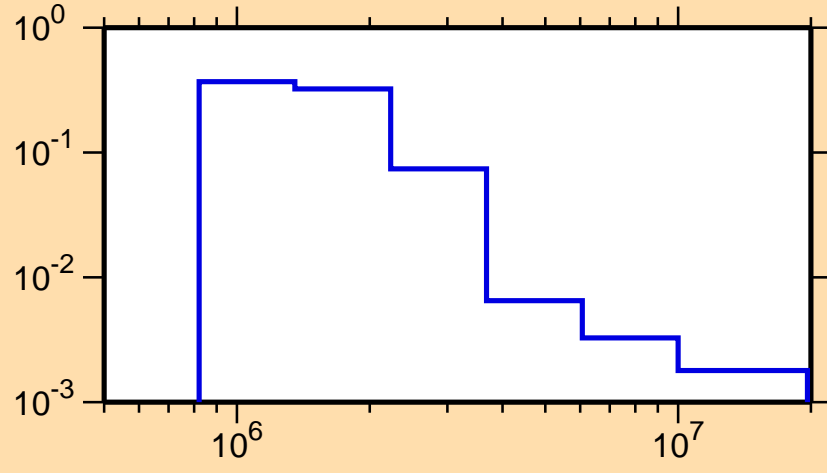
\sigma vs. E for ^{166}\text{Dy}(n,n_4)
