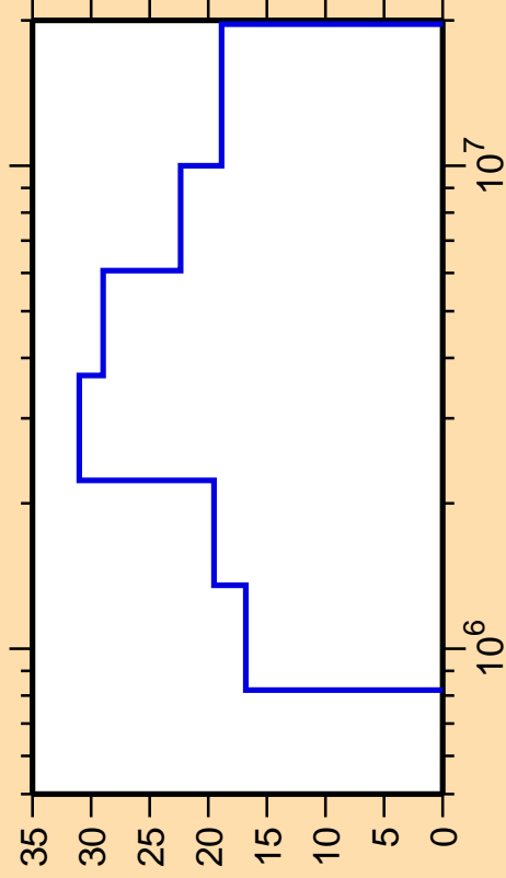
\Delta\sigma/\sigma vs. E for ^{166}\text{Dy}(n,n_4)
