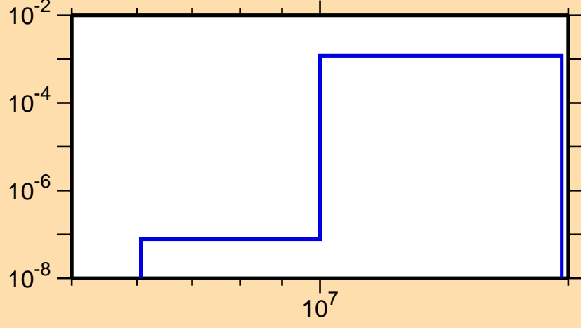
\sigma vs. E for ^{166}\text{Dy}(n,p)
