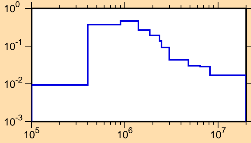
\sigma vs. E for ^{166}\text{Dy}(n,n_2)
