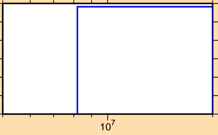
\sigma vs. E for ^{166}\text{Dy}(n,d)
