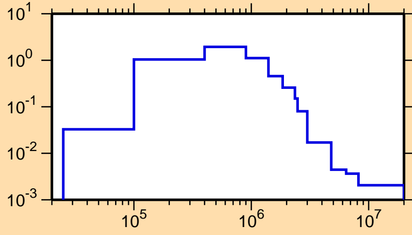
\sigma vs. E for ^{166}\text{Dy}(n,n_1)
