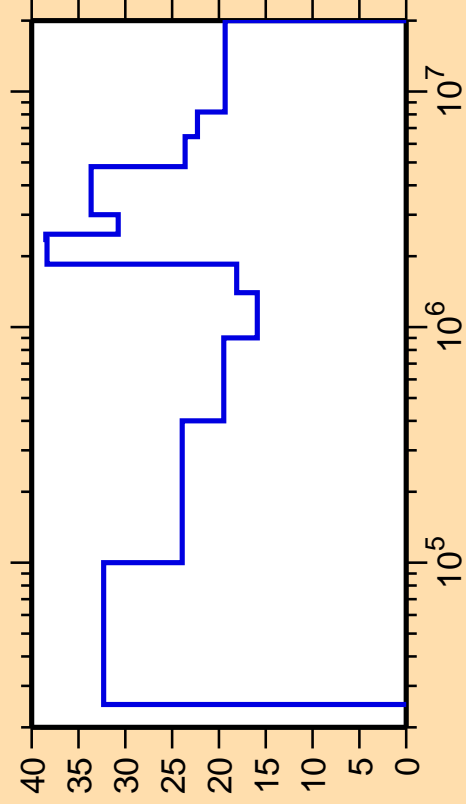
\Delta\sigma/\sigma vs. E for ^{166}\text{Dy}(n,n_1)
