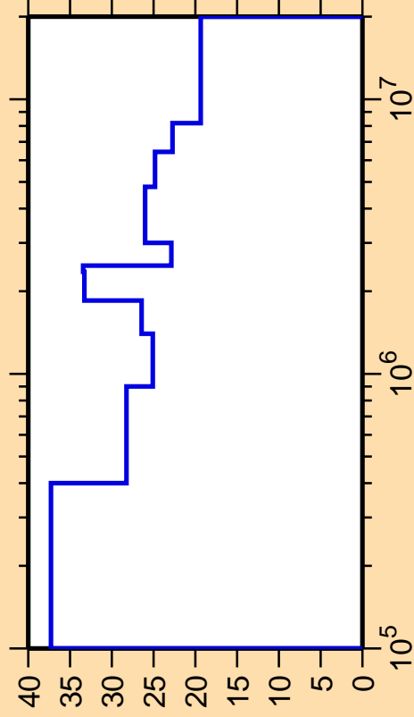
\Delta\sigma/\sigma vs. E for ^{166}\text{Dy}(n,n_2)
