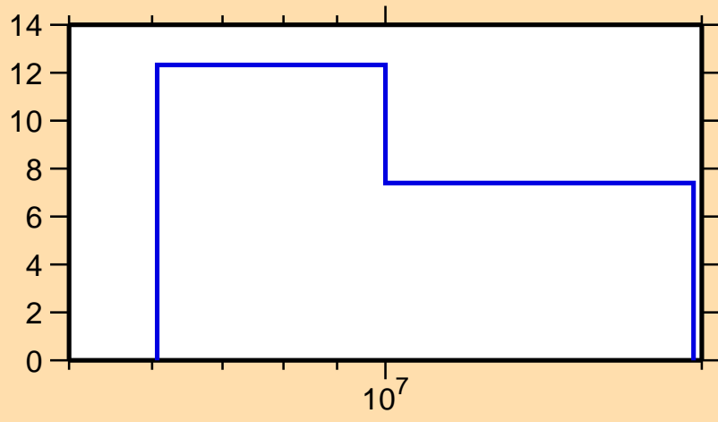
\Delta\sigma/\sigma vs. E for ^{168}\text{Dy}(n,el.)
