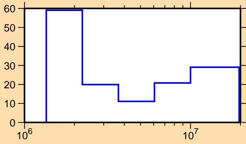
\Delta\sigma/\sigma vs. E for ^{168}\text{Dy}(n,n\text{cont.})
