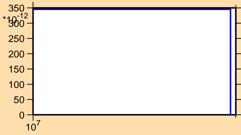
\sigma vs. E for ^{168}\text{Dy}(n,nt)
