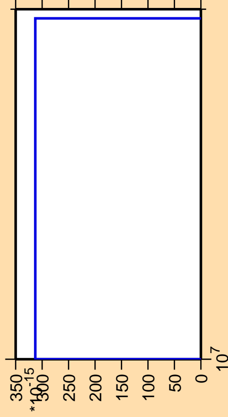
\Delta\sigma/\sigma vs. E for ^{168}\text{Dy} (mt 11)
