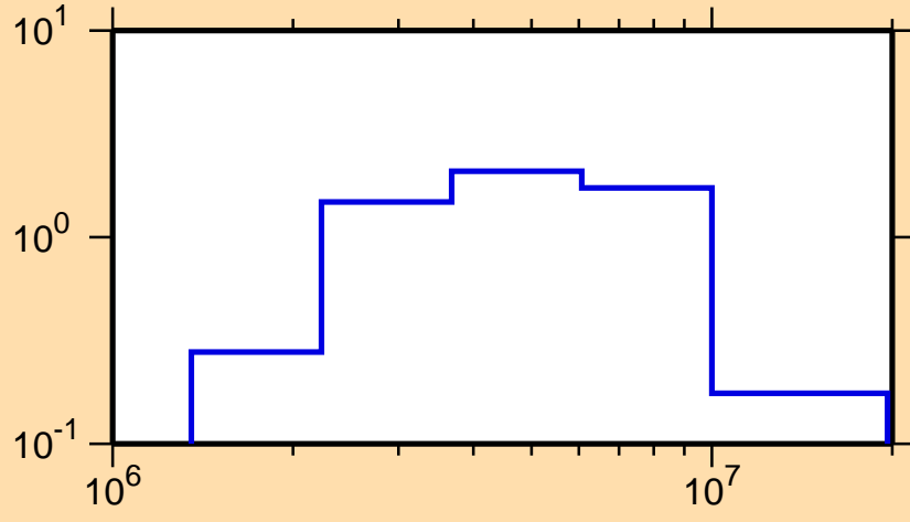
\sigma vs. E for ^{168}\text{Dy}(n,n\text{cont.})
