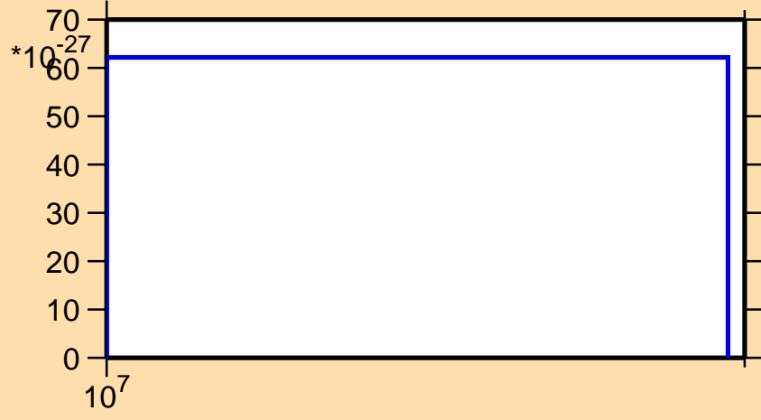
\sigma vs. E for ^{168}\text{Dy} (mt 11)
