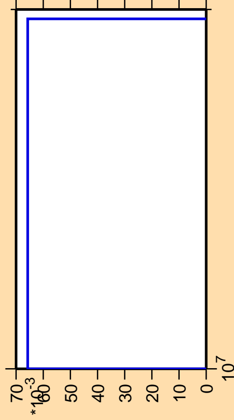
\Delta\sigma/\sigma vs. E for ^{168}\text{Dy}(n,2np)
