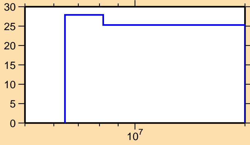
\Delta\sigma/\sigma vs. E for ^{168}\text{Dy}(n,n\text{cont.})
