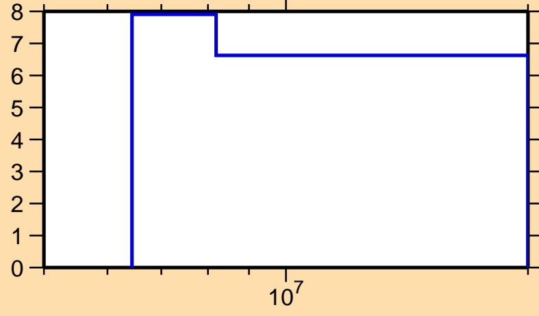
\Delta\sigma/\sigma vs. E for ^{168}\text{Dy}(n,\text{nonel.})
