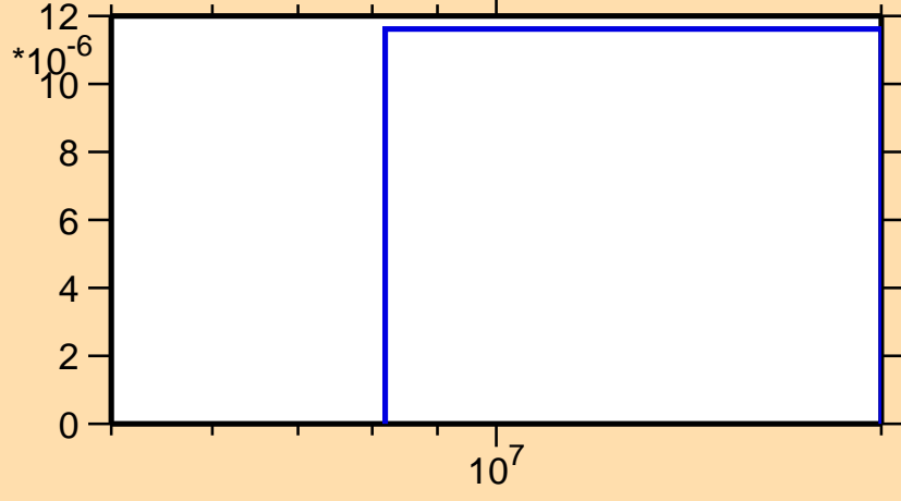
\sigma vs. E for ^{168}\text{Dy}(n,d)
