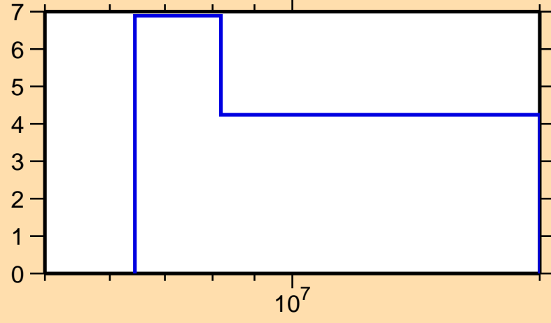
\Delta\sigma/\sigma vs. E for ^{168}\text{Dy}(n,\text{tot.})
