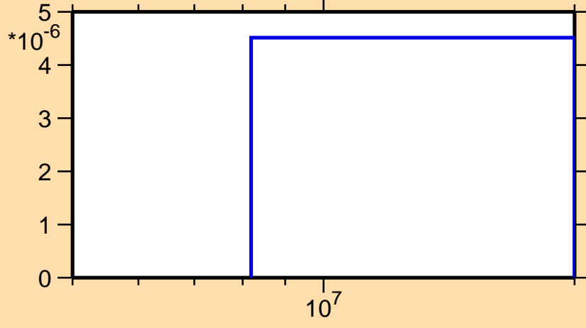
\sigma vs. E for ^{168}\text{Dy}(n,t)
