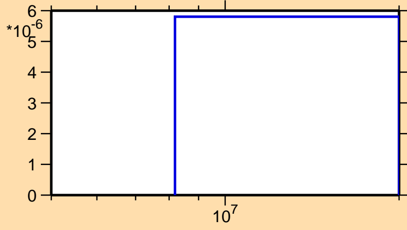
\sigma vs. E for ^{168}\text{Dy}(n,np)
