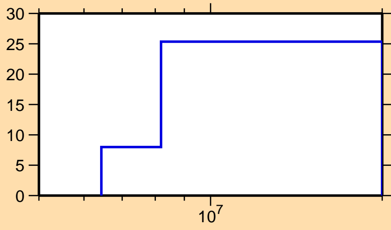
\Delta\sigma/\sigma vs. E for ^{168}\text{Dy}(n,p)
