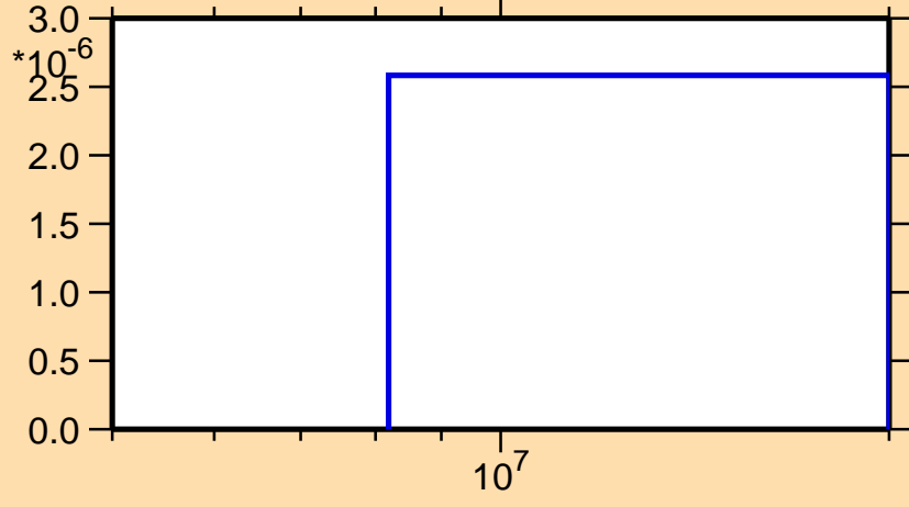
\sigma vs. E for ^{168}\text{Dy}(n,n\alpha)
