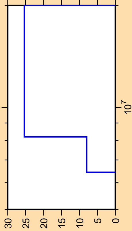
\Delta\sigma/\sigma vs. E for ^{168}\text{Dy}(n,p)
