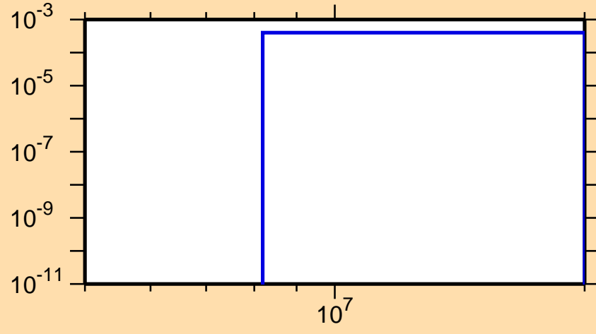
\sigma vs. E for ^{168}\text{Dy}(n,p)
