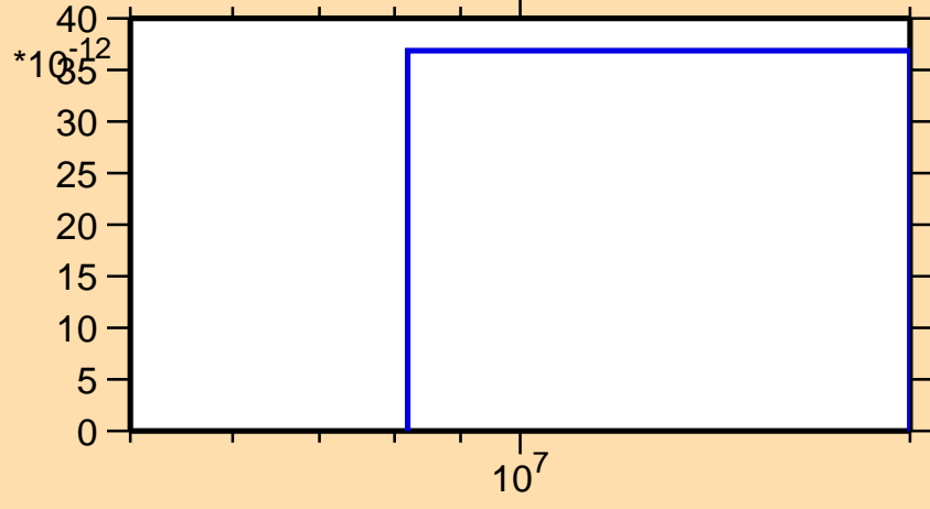
\sigma vs. E for ^{168}\text{Dy}(n,nd)
