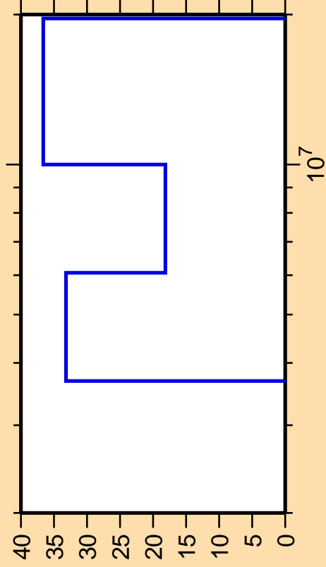
\Delta\sigma/\sigma vs. E for ^{169}\text{Dy}(n,2n)
