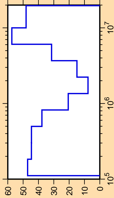
\Delta\sigma/\sigma vs. E for ^{169}\text{Dy}(n,\text{inel.})
