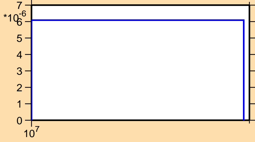
\sigma vs. E for ^{169}\text{Dy}(n,np)
