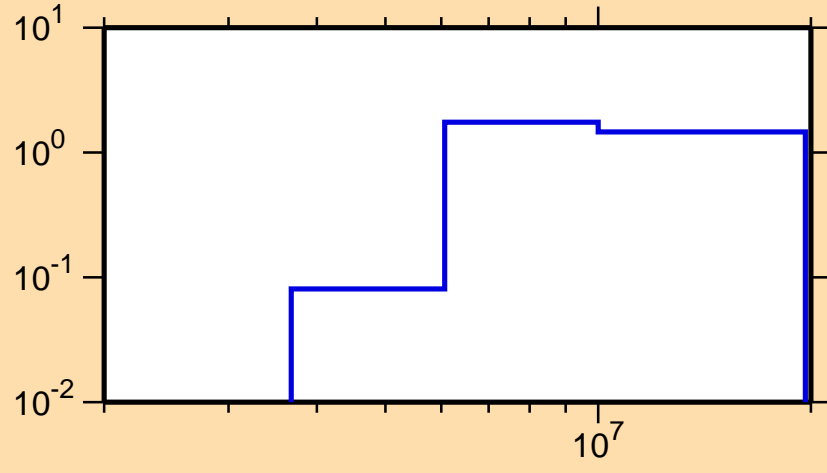
\sigma vs. E for ^{169}\text{Dy}(n,2n)
