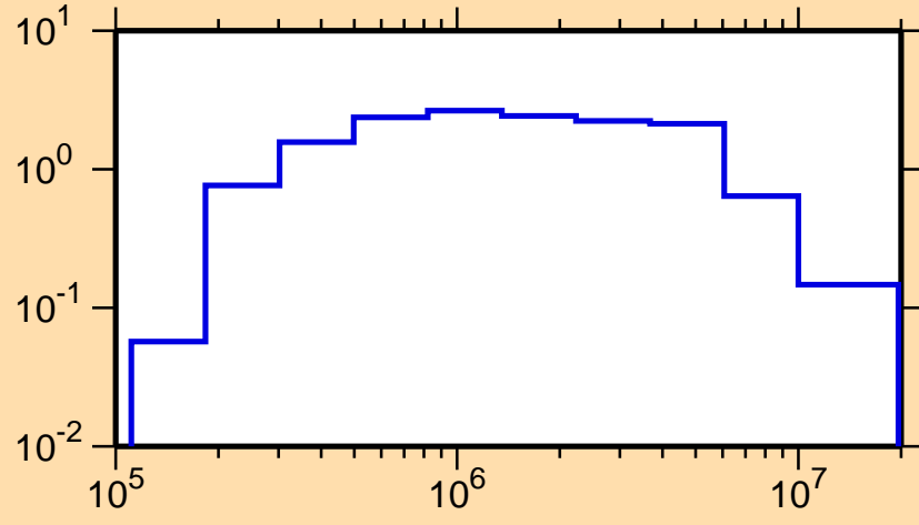
\sigma vs. E for ^{169}\text{Dy}(n,\text{inel.})
