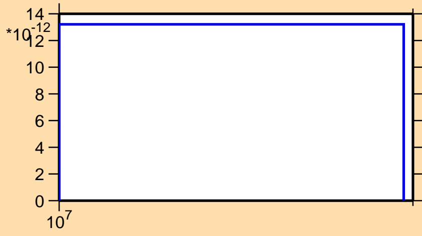
\sigma vs. E for ^{169}\text{Dy}(n,2np)
