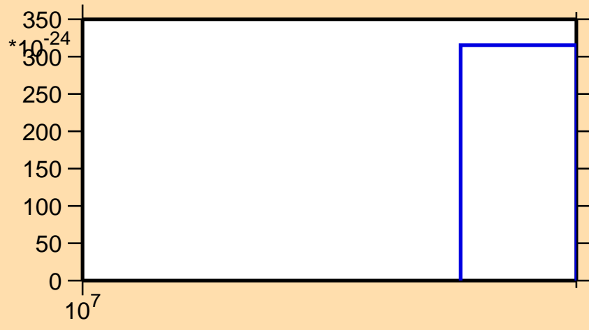
\sigma vs. E for ^{170}\text{Dy} (mt 11)
