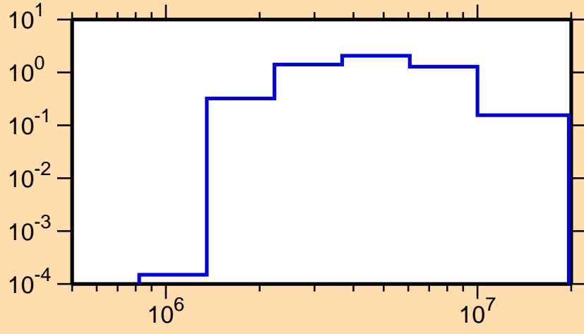
\sigma vs. E for ^{170}\text{Dy}(n,n\text{cont.})
