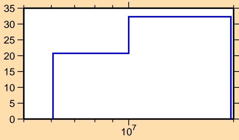
\Delta\sigma/\sigma vs. E for ^{170}\text{Dy}(n,n\text{cont.})
