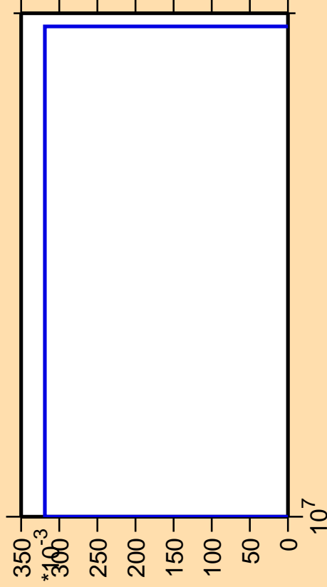
\Delta\sigma/\sigma vs. E for ^{170}\text{Dy}(n,2np)
