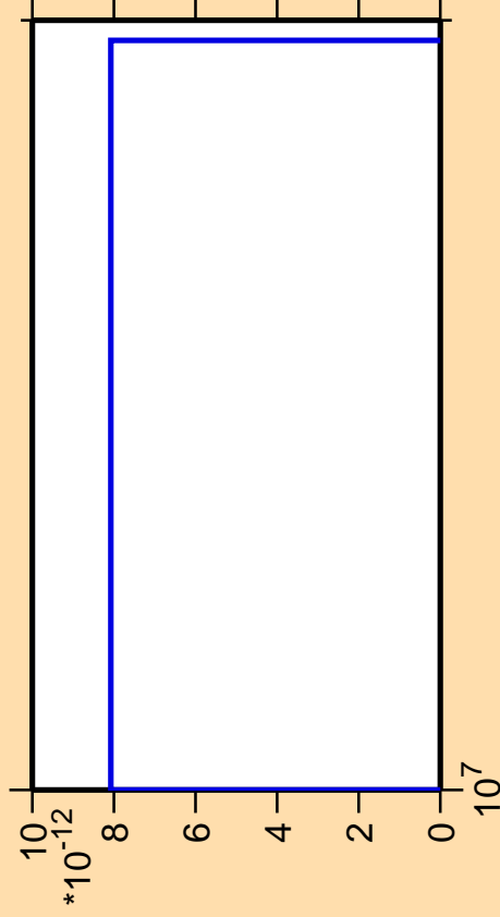
\Delta\sigma/\sigma vs. E for ^{170}\text{Dy} (mt 11)
