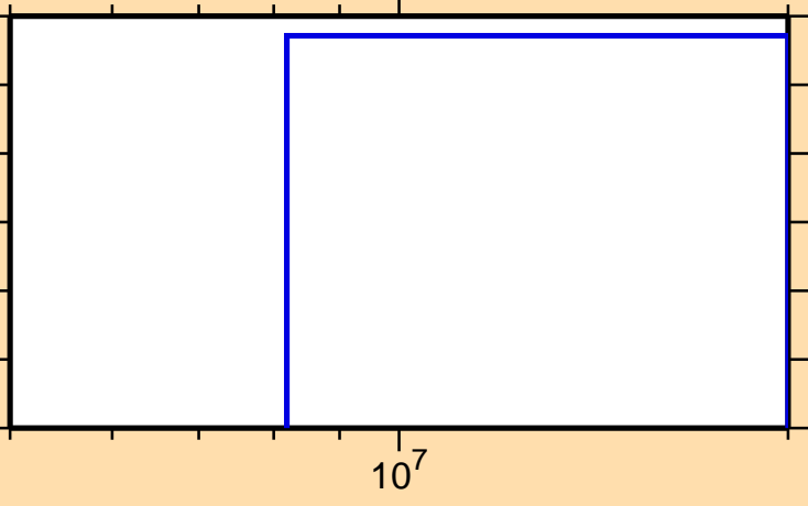
\sigma vs. E for ^{170}\text{Dy}(n,nt)
