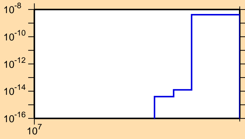
\sigma vs. E for ^{171}\text{Dy}(n,2np)
