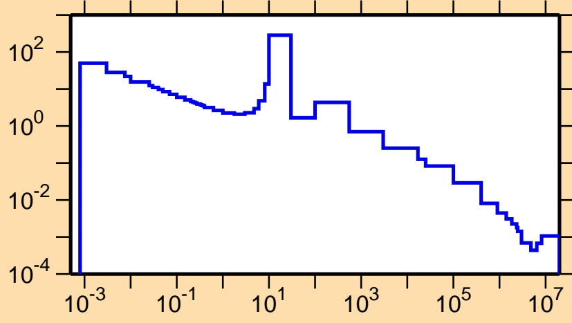
\sigma vs. E for ^{171}\text{Dy}(n,\gamma)
