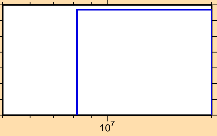
\sigma vs. E for ^{171}\text{Dy}(n,t)
