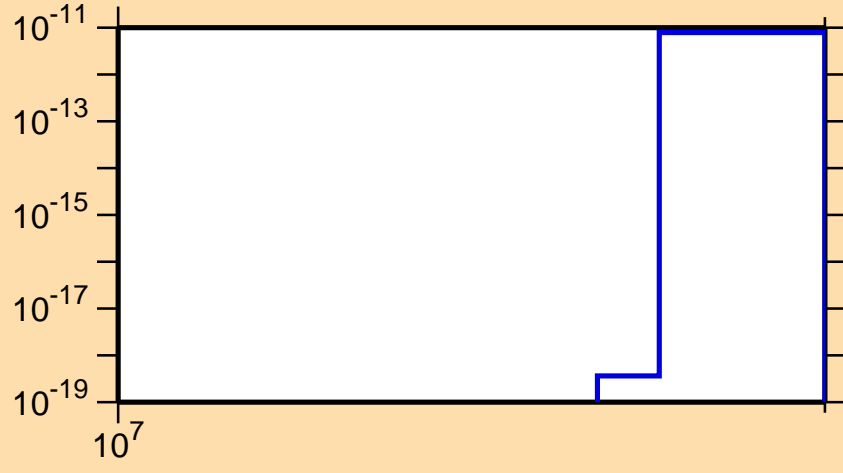
\sigma vs. E for ^{172}\text{Dy}(n,2np)
