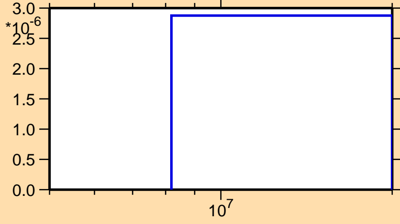
\sigma vs. E for ^{172}\text{Dy}(n,t)
