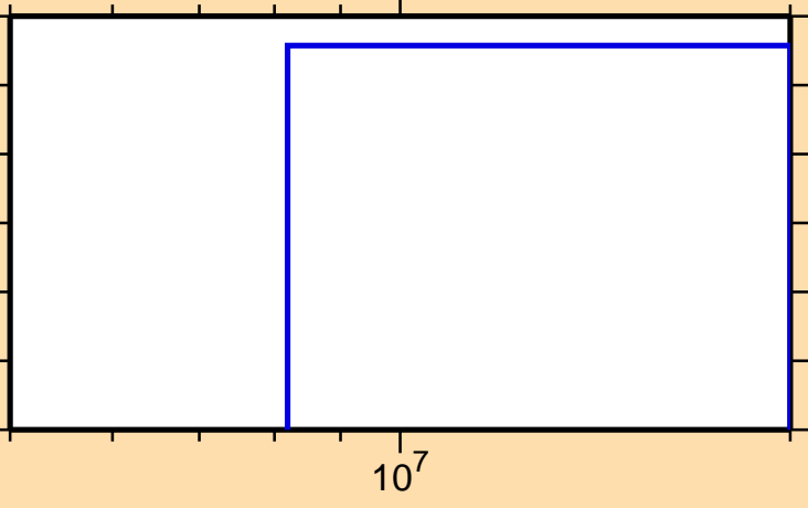
\sigma vs. E for ^{172}\text{Dy}(n,n\alpha)
