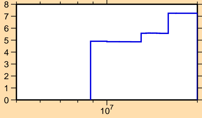
\Delta\sigma/\sigma vs. E for ^{173}\text{Dy}(n,el.)
