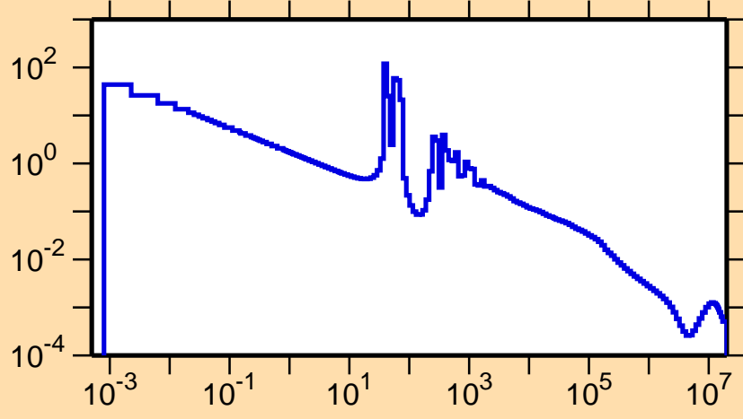
\sigma vs. E for ^{173}\text{Dy}(n,\gamma)
