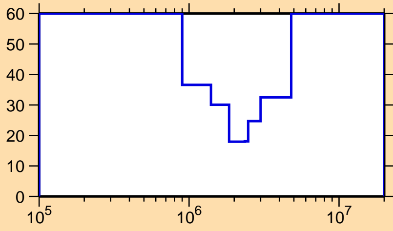
\Delta\sigma/\sigma vs. E for ^{173}\text{Dy}(n,n\text{cont.})
