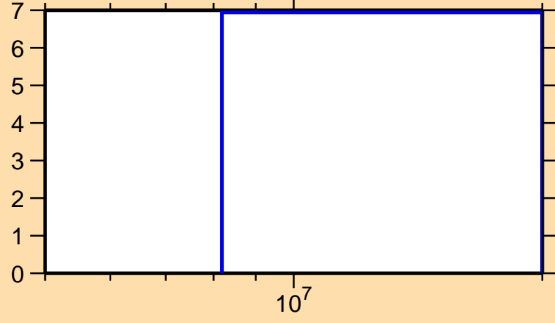
\Delta\sigma/\sigma vs. E for ^{146}\text{Er}(n,\text{el.})
