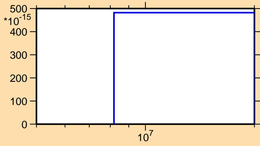
\sigma vs. E for ^{146}\text{Er}(n,2n\alpha)
