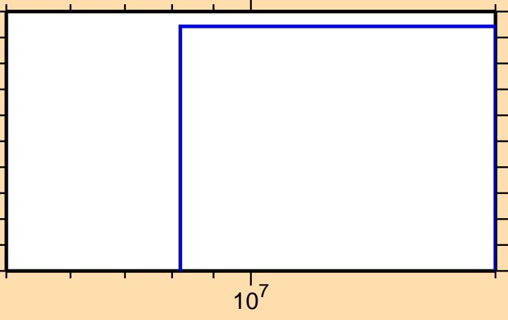
\sigma vs. E for ^{146}\text{Er}(n,t)
