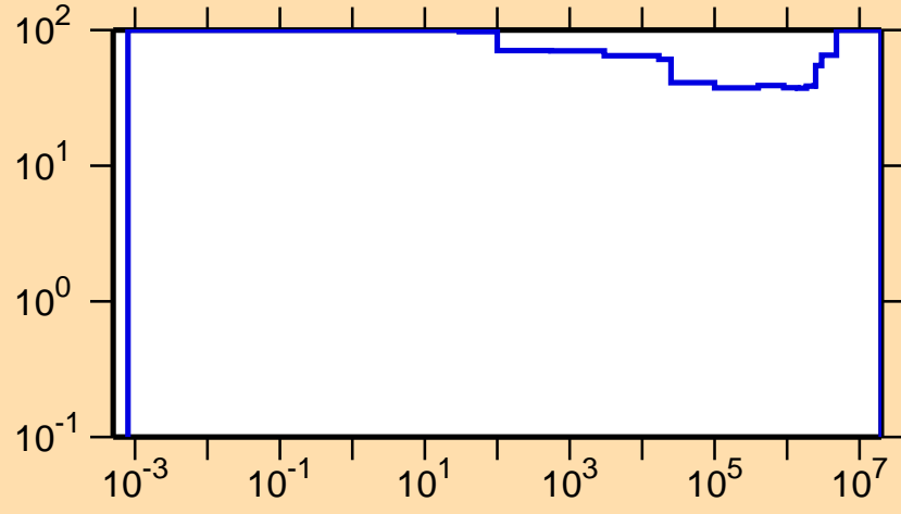
\Delta\sigma/\sigma vs. E for ^{146}\text{Er}(n,p)
