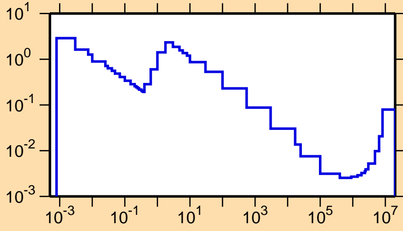
\sigma vs. E for ^{146}\text{Er}(n,\alpha)
