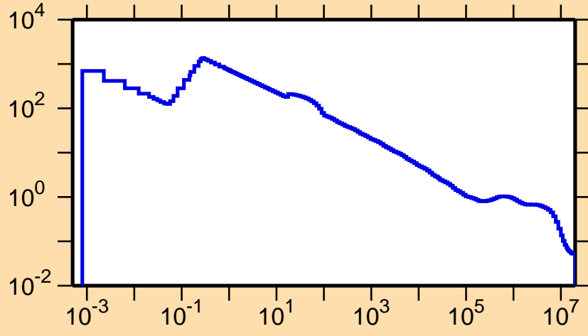
\sigma vs. E for ^{147}\text{Er}(n,p)
