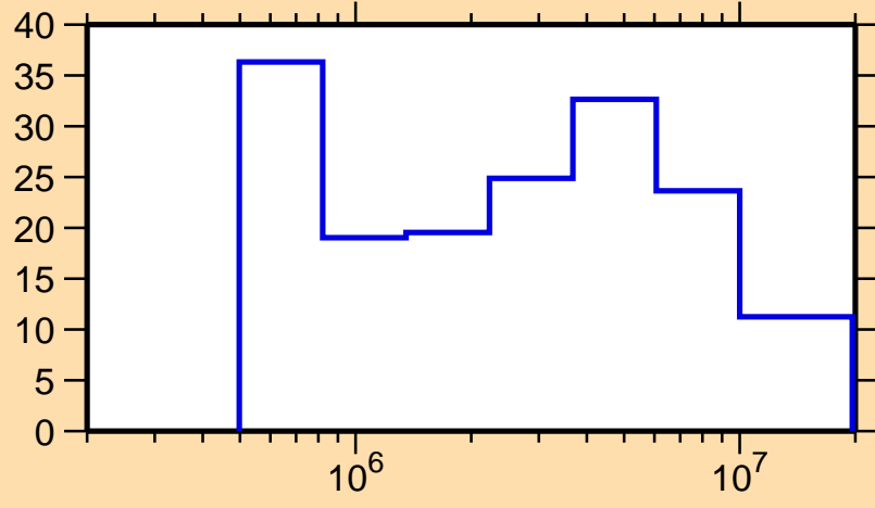
\Delta\sigma/\sigma vs. E for ^{147}\text{Er}(n, el.)
