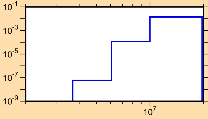
\sigma vs. E for ^{147}\text{Er}(n,d)
