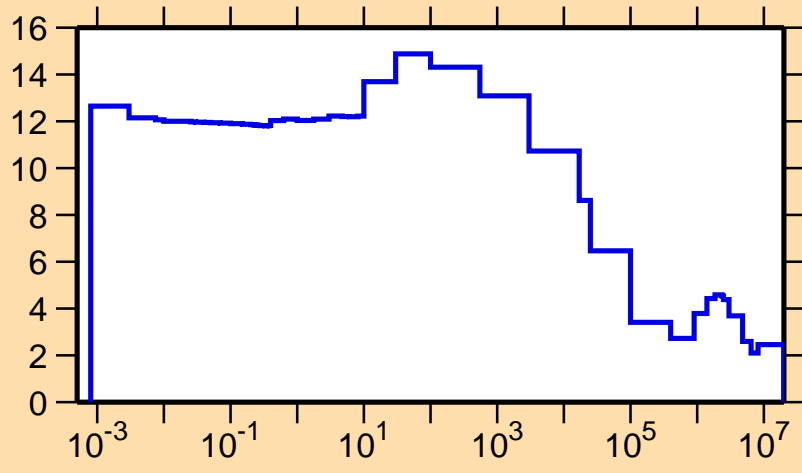
\sigma vs. E for ^{147}\text{Er}(n,\text{el.})
