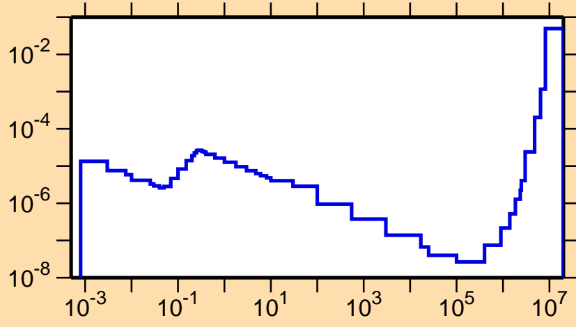
\sigma vs. E for ^{147}\text{Er}(n,p\alpha)
