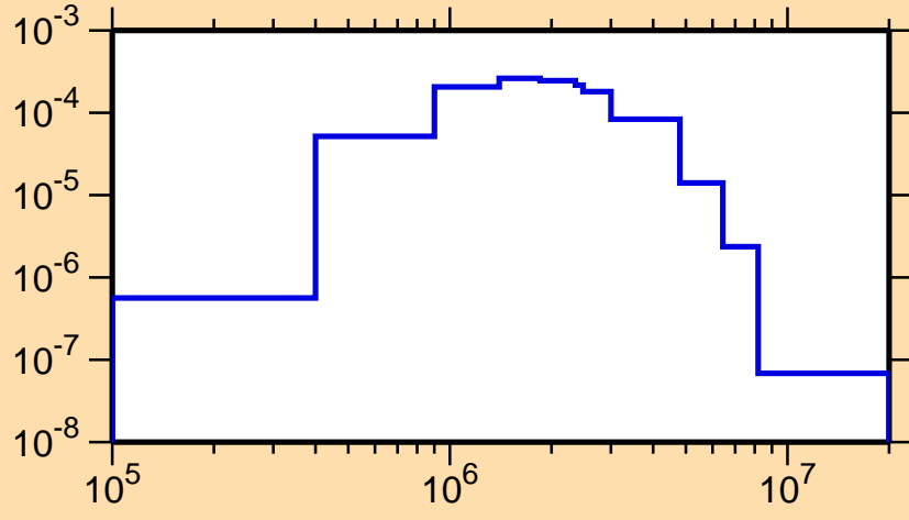
\sigma vs. E for ^{147}\text{Er}(n,n_2)
