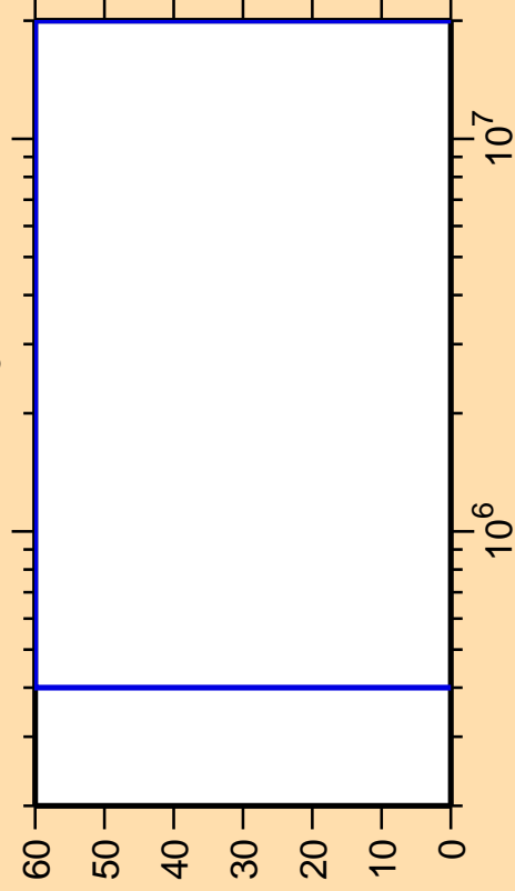
\Delta\sigma/\sigma vs. E for ^{147}\text{Er}(n,n_3)
