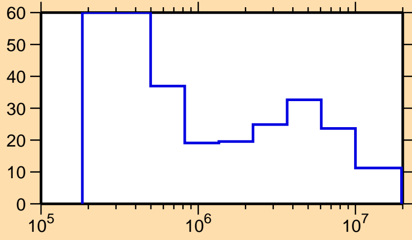
\Delta\sigma/\sigma vs. E for ^{147}\text{Er}(n, el.)
