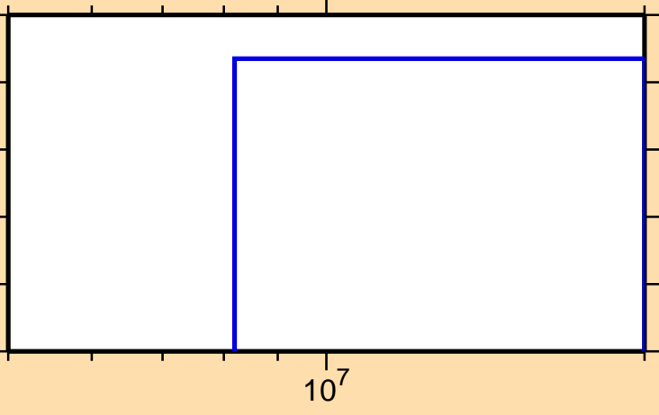
\sigma vs. E for ^{147}\text{Er}(n,2np)
