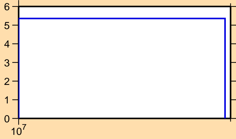
\Delta\sigma/\sigma vs. E for ^{148}\text{Er}(n,\text{el.})
