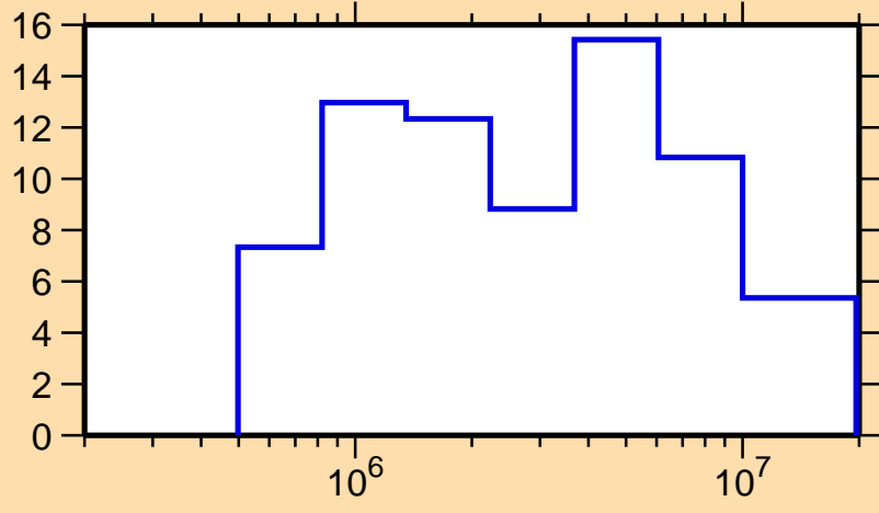
\Delta\sigma/\sigma vs. E for ^{148}\text{Er}(n,\text{el.})
