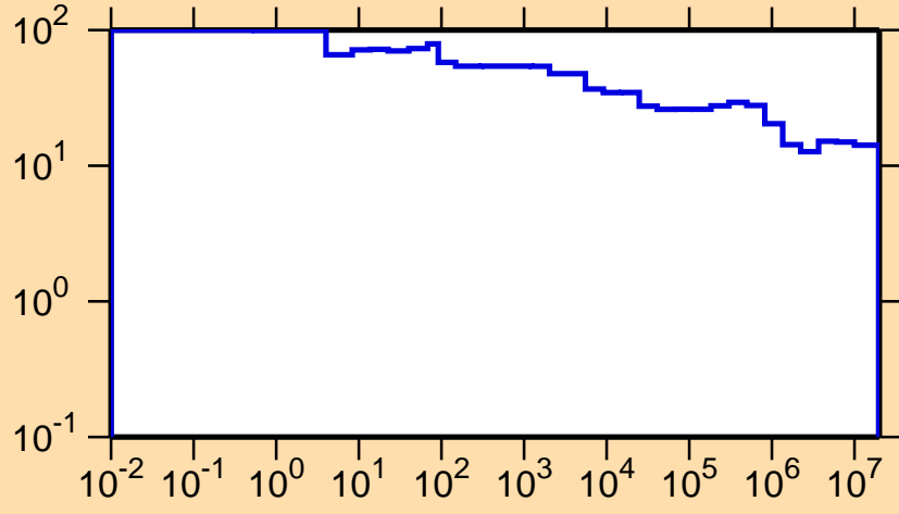
\Delta\sigma/\sigma vs. E for ^{148}\text{Er}(n,\text{nonel.})
