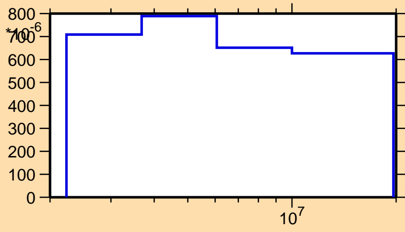
\sigma vs. E for ^{148}\text{Er}(n,n_3)
