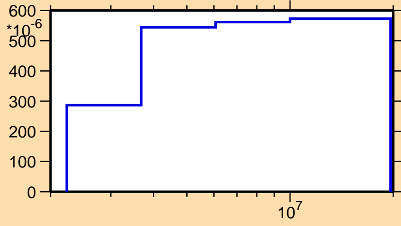
\sigma vs. E for ^{148}\text{Er}(n,n_4)
