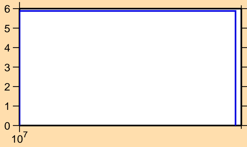
\Delta\sigma/\sigma vs. E for ^{148}\text{Er}(n,\text{tot.})
