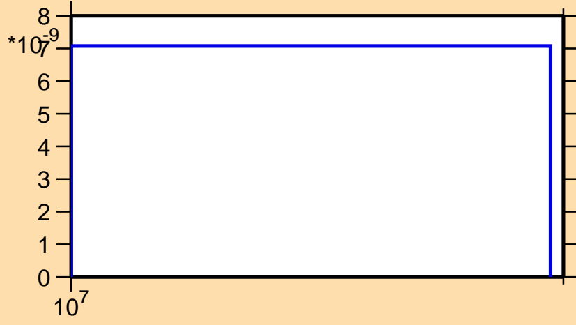
\sigma vs. E for ^{148}\text{Er}(n,\text{pt})
