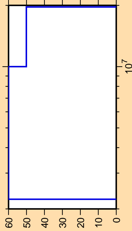
\Delta\sigma/\sigma vs. E for ^{148}\text{Er}(n,n_4)
