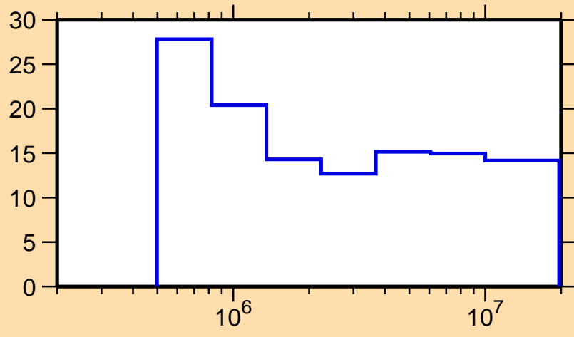
\Delta\sigma/\sigma vs. E for ^{148}\text{Er}(n,\text{nonel.})
