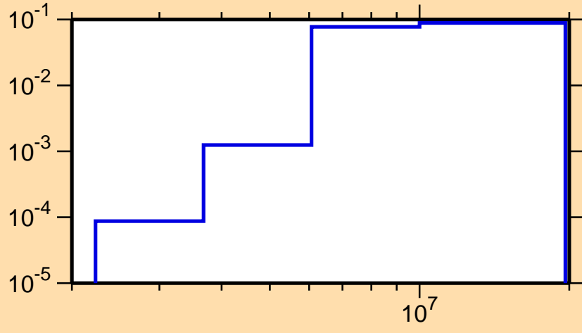
\sigma vs. E for ^{148}\text{Er}(n,n\text{cont.})
