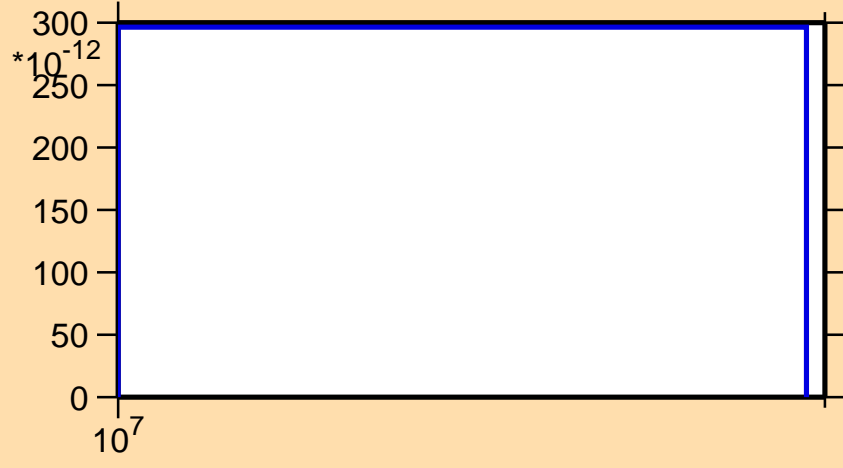
\sigma vs. E for ^{148}\text{Er}(\text{mt117})
