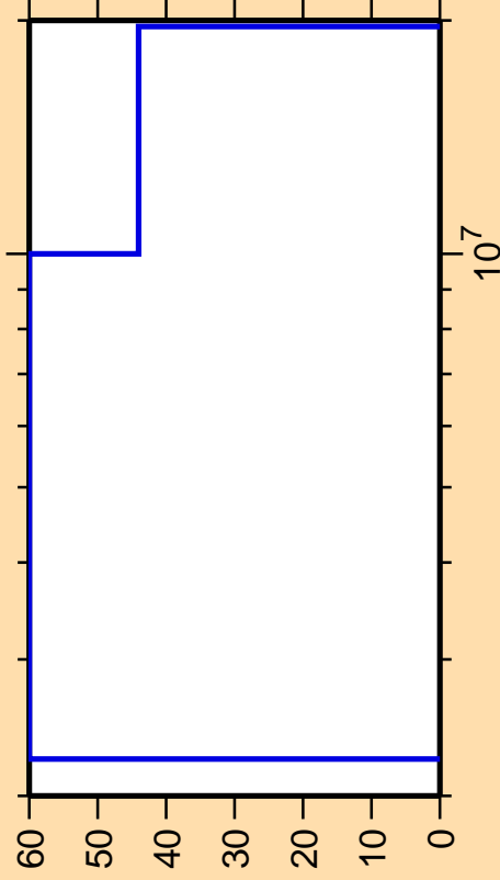
\Delta\sigma/\sigma vs. E for ^{148}\text{Er}(n,n\text{cont.})
