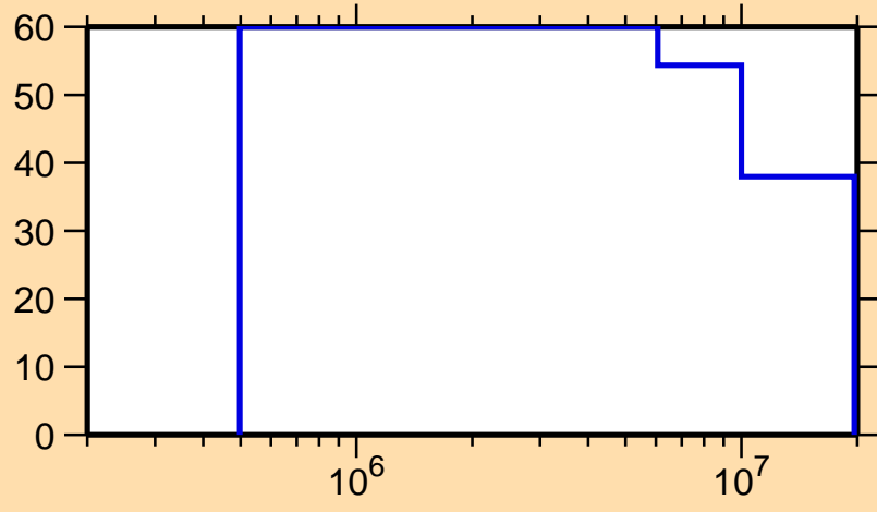
\Delta\sigma/\sigma vs. E for ^{148}\text{Er}(n,\text{inel.})
