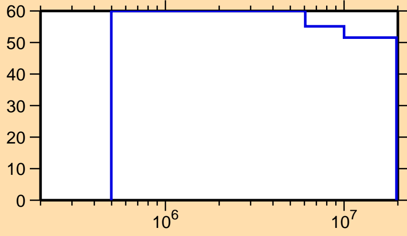
\Delta\sigma/\sigma vs. E for ^{148}\text{Er}(n,n_1)
