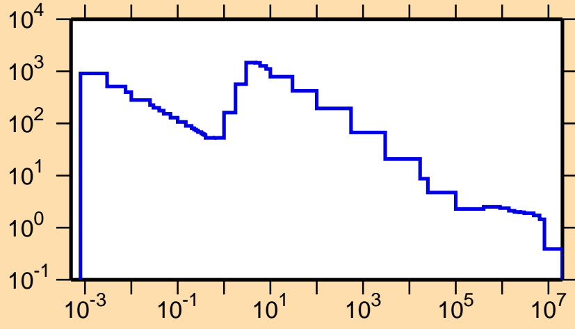
\sigma vs. E for ^{148}\text{Er}(n,p)
