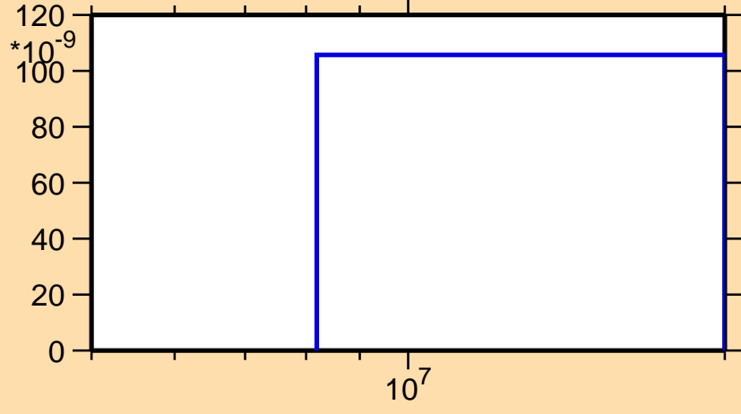
\sigma vs. E for ^{148}\text{Er} (mt 45)
