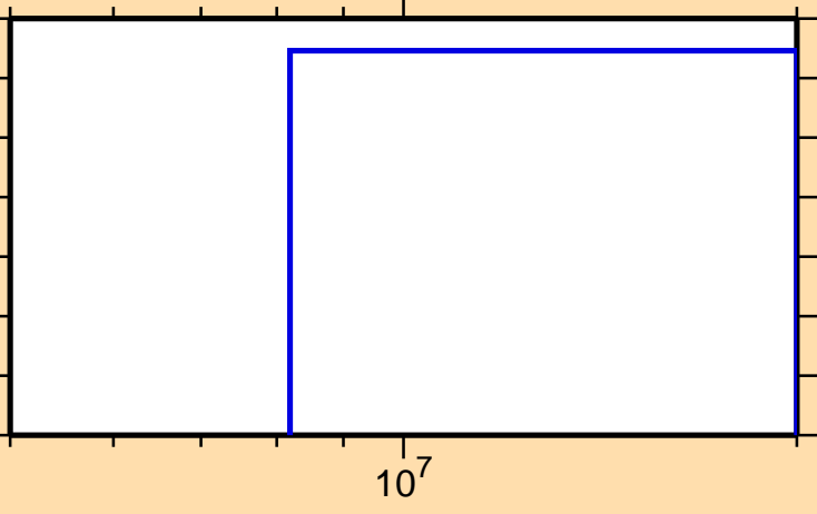
\sigma vs. E for ^{148}\text{Er}(n,\text{pt})
