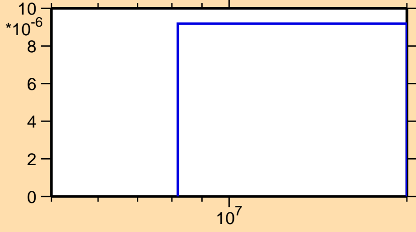
\sigma vs. E for ^{148}\text{Er}(n,t)
