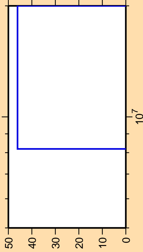
\Delta\sigma/\sigma vs. E for ^{148}\text{Er} (mt 45)
