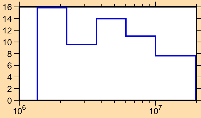
\Delta\sigma/\sigma vs. E for ^{149}\text{Er}(n, el.)
