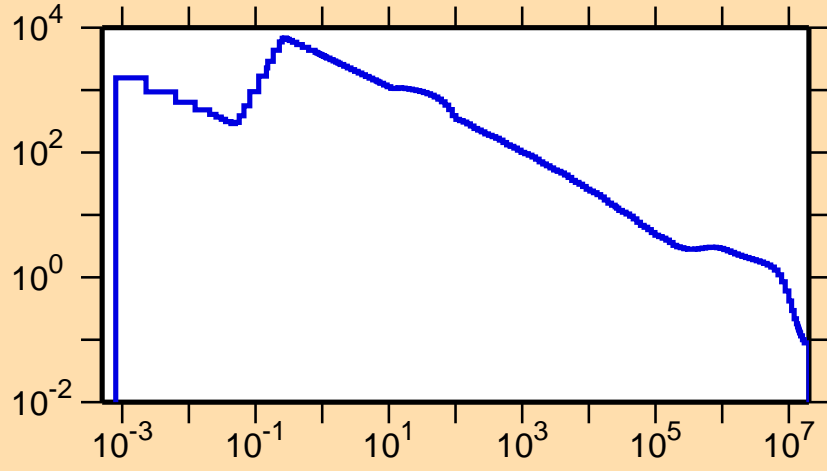
\sigma vs. E for ^{149}\text{Er}(n,p)
