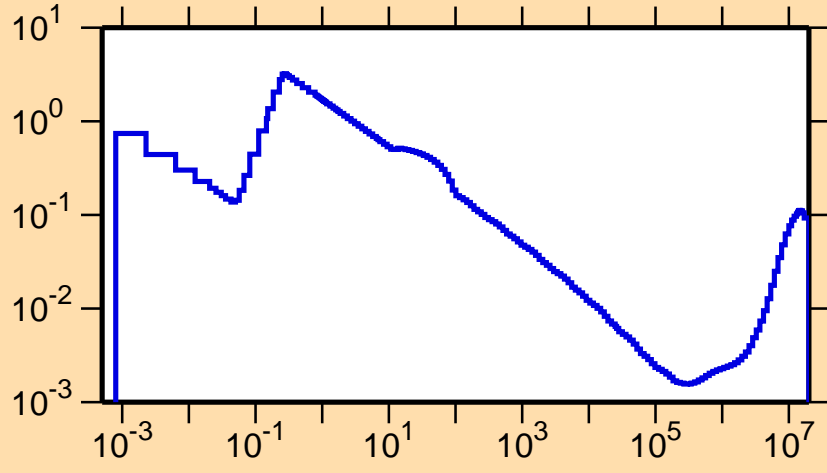
\sigma vs. E for ^{149}\text{Er}(n,\alpha)
