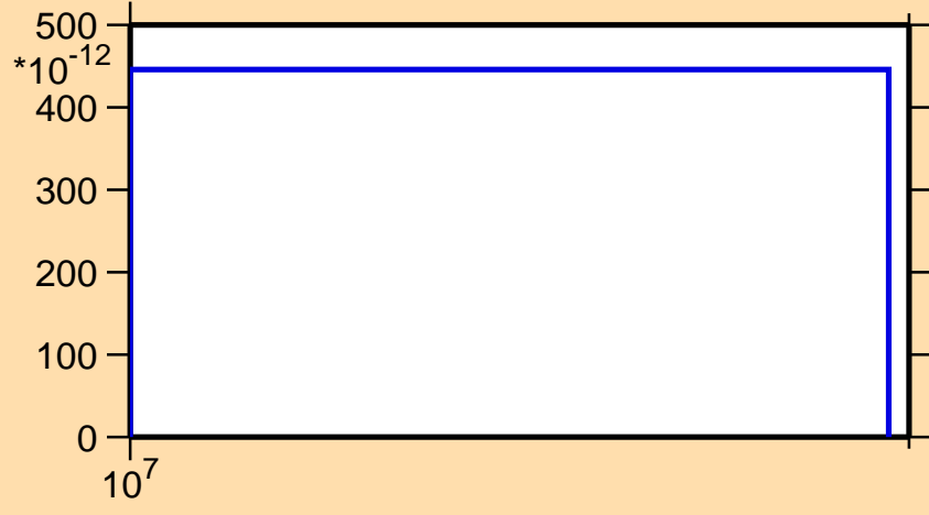
\sigma vs. E for ^{150}\text{Er}(\text{mt117})
