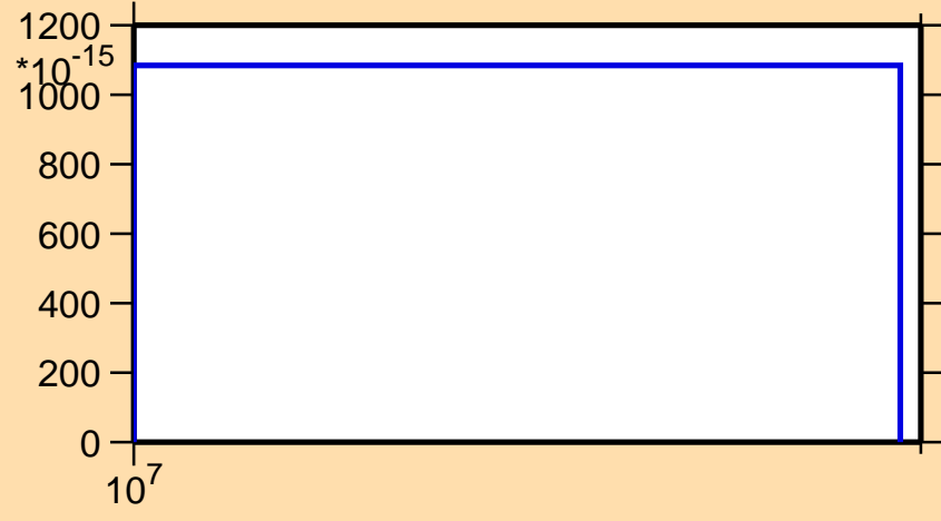
\sigma vs. E for ^{150}\text{Er} (mt 34)
