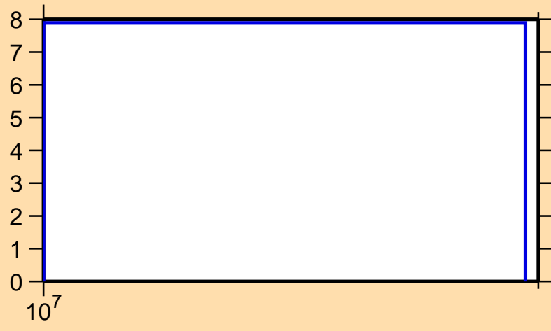
\Delta\sigma/\sigma vs. E for ^{150}\text{Er}(n,\text{nonel.})
