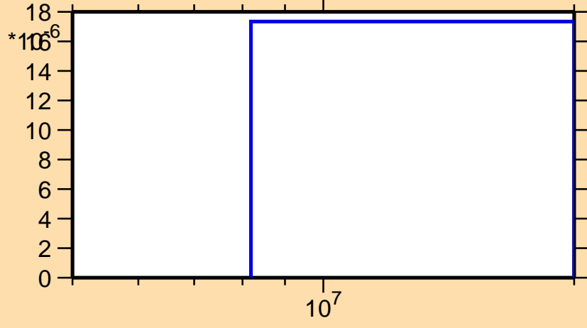
\sigma vs. E for ^{150}\text{Er}(n,t)
