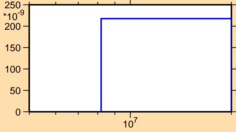
\sigma vs. E for ^{150}\text{Er}(\text{mt } 45)
