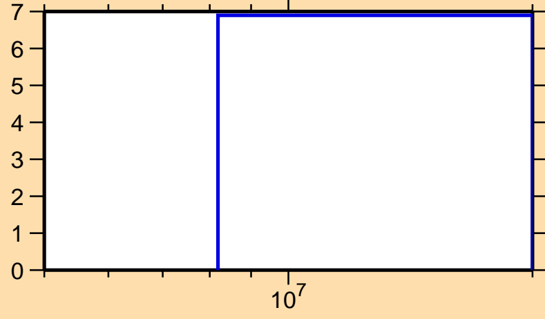
\Delta\sigma/\sigma vs. E for ^{150}\text{Er}(n,\text{el.})
