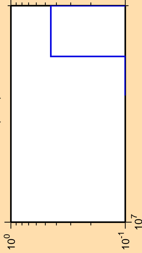
\Delta\sigma/\sigma vs. E for ^{151}\text{Er}(n,nt)
