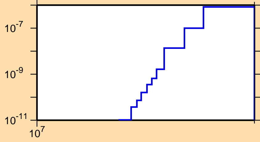
\sigma vs. E for ^{151}\text{Er}(n,2n\alpha)
