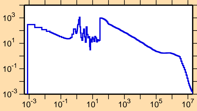
\sigma vs. E for ^{151}\text{Er}(n,\gamma)
