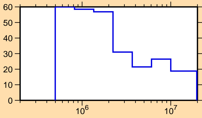
\Delta\sigma/\sigma vs. E for ^{151}\text{Er}(n,n_1)
