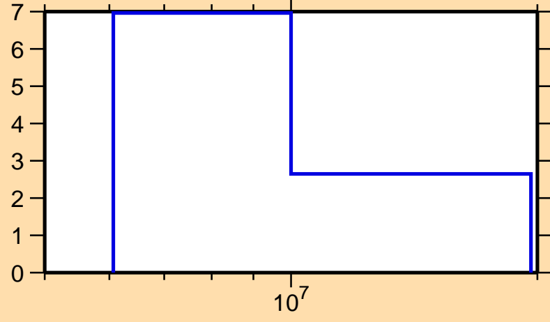
\Delta\sigma/\sigma vs. E for ^{151}\text{Er}(n,\text{tot.})
