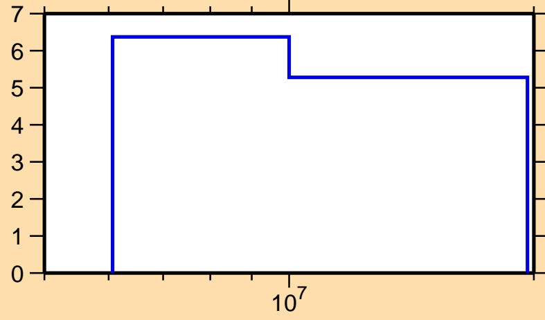
\Delta\sigma/\sigma vs. E for ^{151}\text{Er}(n,\text{nonel.})
