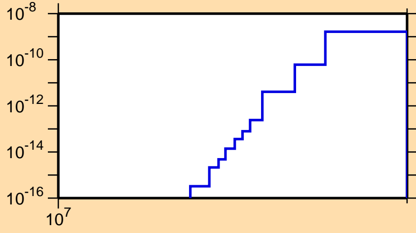
\sigma vs. E for ^{152}\text{Er}(\text{mt } 34)
