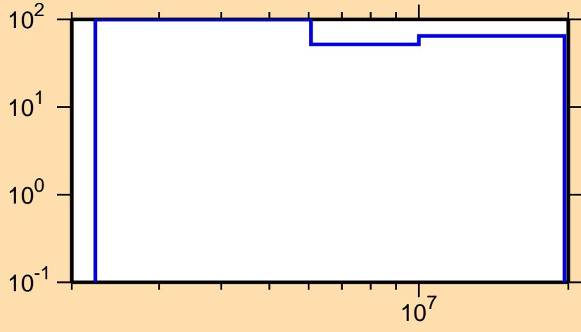
\Delta\sigma/\sigma vs. E for ^{152}\text{Er}(n,n\text{cont.})
