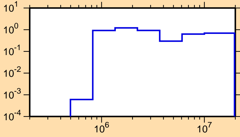
\sigma vs. E for ^{152}\text{Er}(n,\text{inel.})
