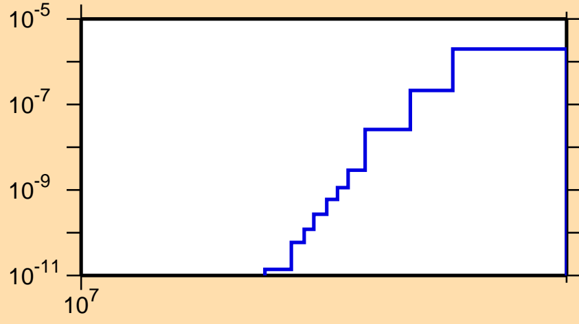
\sigma vs. E for ^{153}\text{Er}(n,\text{pt})
