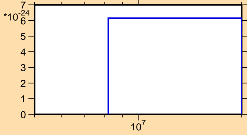
\sigma vs. E for ^{153}\text{Er}(\text{mt } 11)
