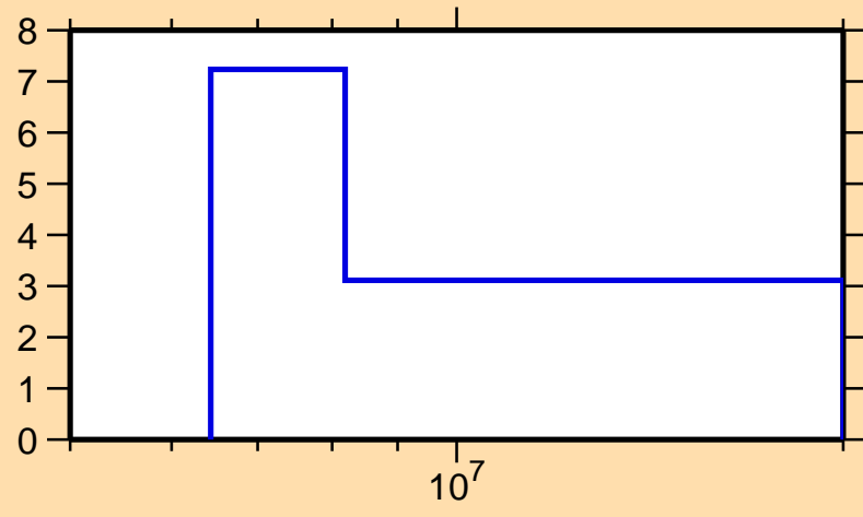
\Delta\sigma/\sigma vs. E for ^{153}\text{Er}(n,\text{tot.})
