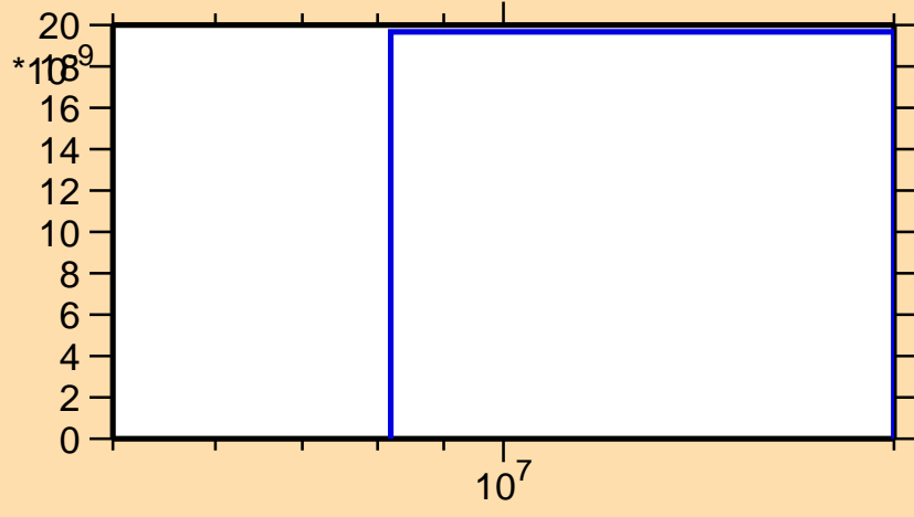
\sigma vs. E for ^{153}\text{Er}(\text{mt117})
