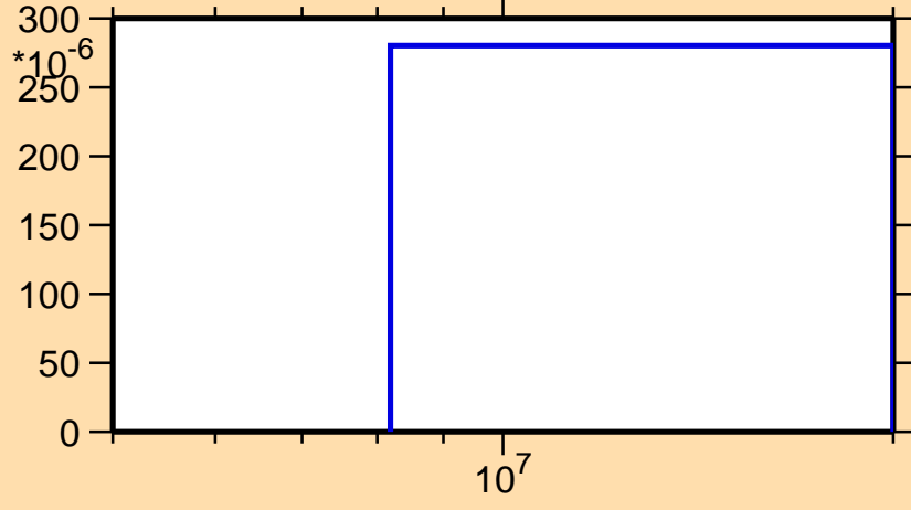
\sigma vs. E for ^{153}\text{Er}(n,2n\alpha)
