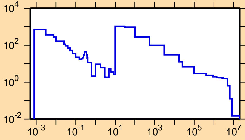
\sigma vs. E for ^{153}\text{Er}(n,\gamma)
