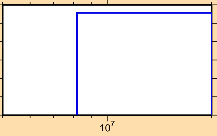
\sigma vs. E for ^{153}\text{Er}(n,\text{pt})
