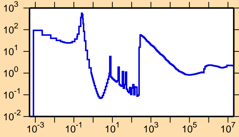
\sigma vs. E for ^{154}\text{Er}(n,\text{nonel.})
