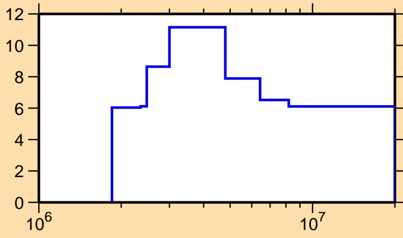
\Delta\sigma/\sigma vs. E for ^{154}\text{Er}(n,\text{nonel.})
