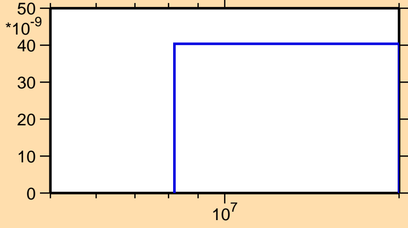
\sigma vs. E for ^{154}\text{Er}(n,\text{pd})
