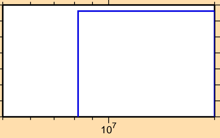
\sigma vs. E for ^{154}\text{Er}(n,\text{nd})
