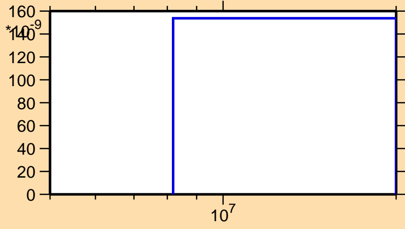
\sigma vs. E for ^{154}\text{Er} (mt 45)
