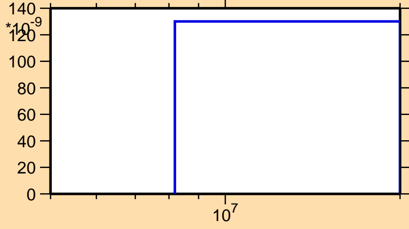
\sigma vs. E for ^{154}\text{Er}(n,2np)
