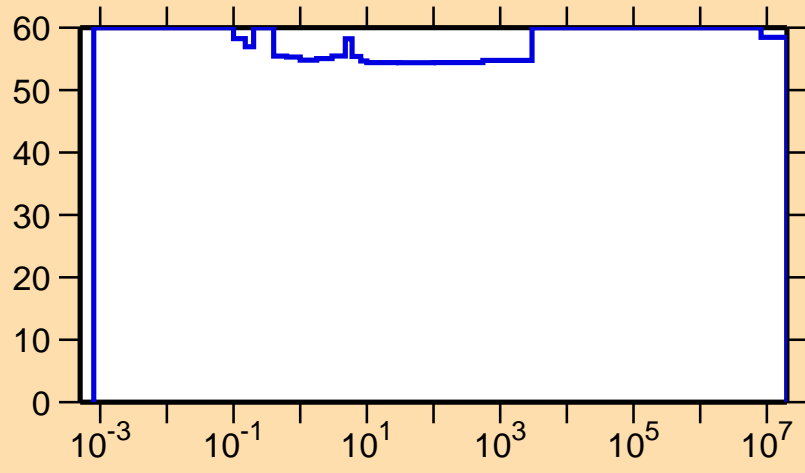
\Delta\sigma/\sigma vs. E for ^{155}\text{Er}(n,p)
