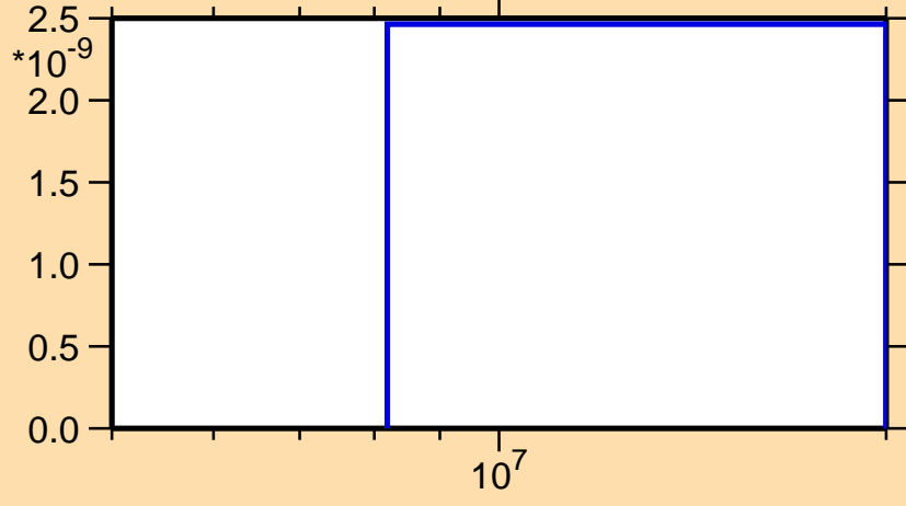
\sigma vs. E for ^{155}\text{Er}(\text{mt } 45)
