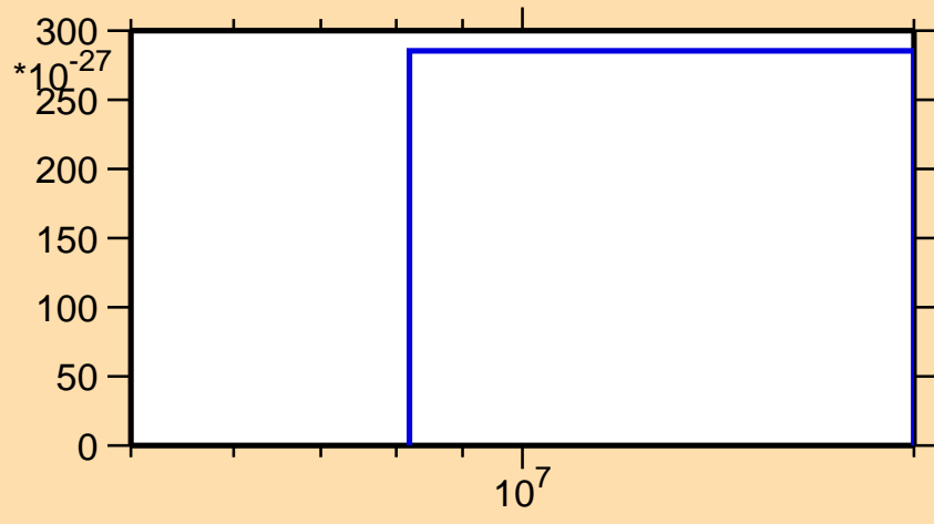
\sigma vs. E for ^{155}\text{Er} (mt 11)
