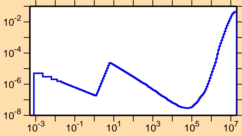
\sigma vs. E for ^{156}\text{Er}(n,p)
