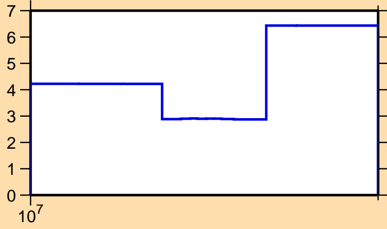
\Delta\sigma/\sigma vs. E for ^{156}\text{Er}(n,\text{el.})
