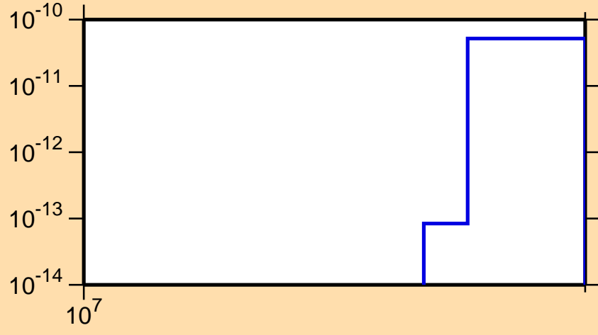
\sigma vs. E for ^{156}\text{Er}(n,\text{pt})
