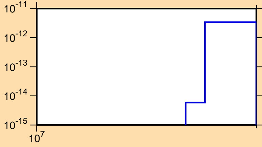
\sigma vs. E for ^{156}\text{Er}(\text{mt } 34)
