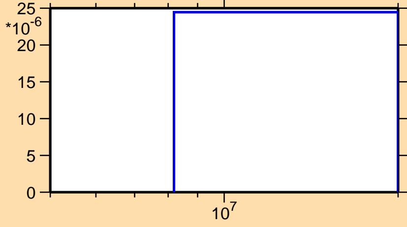
\sigma vs. E for ^{156}\text{Er}(n,t)
