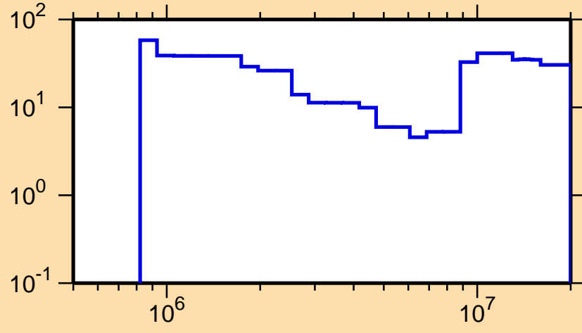
\Delta\sigma/\sigma vs. E for ^{157}\text{Er}(n,n\text{cont.})
