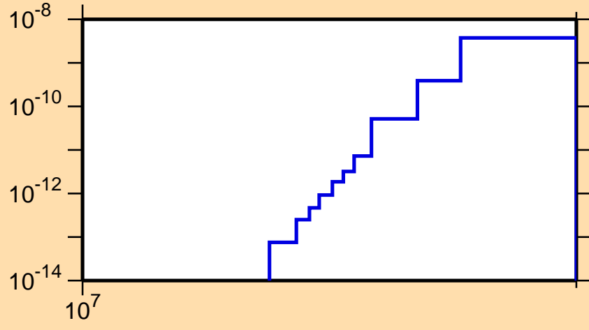
\sigma vs. E for ^{157}\text{Er} (mt 45)
