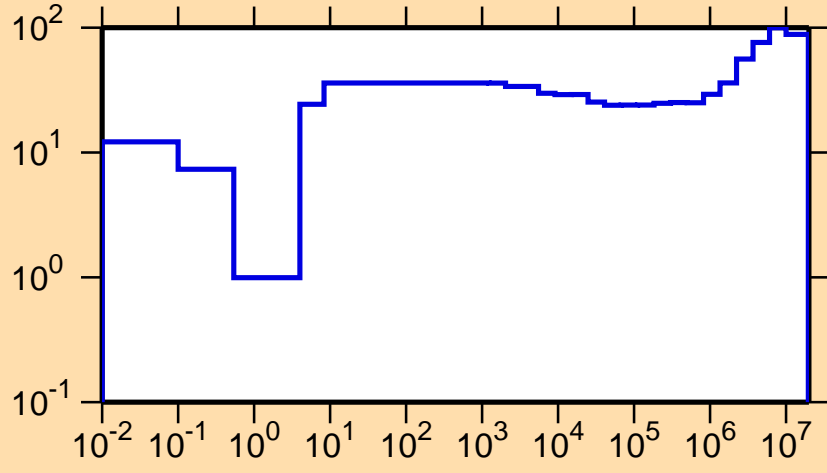
\Delta\sigma/\sigma vs. E for ^{157}\text{Er}(n,\gamma)
