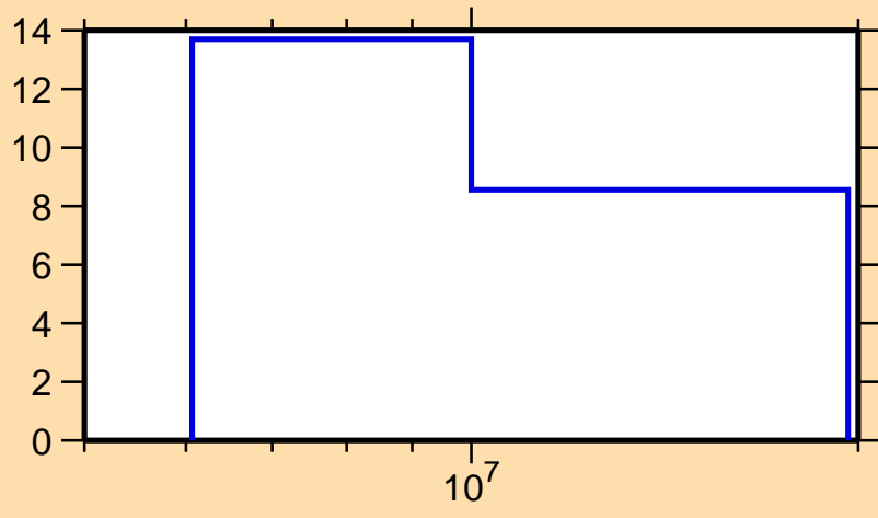
\Delta\sigma/\sigma vs. E for ^{157}\text{Er}(n,2n)
