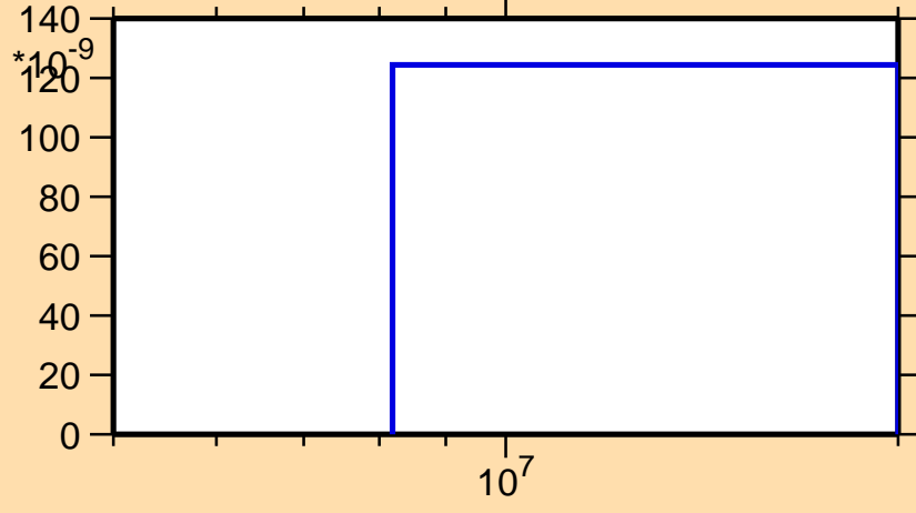
\sigma vs. E for ^{157}\text{Er}(n,\text{He3})
