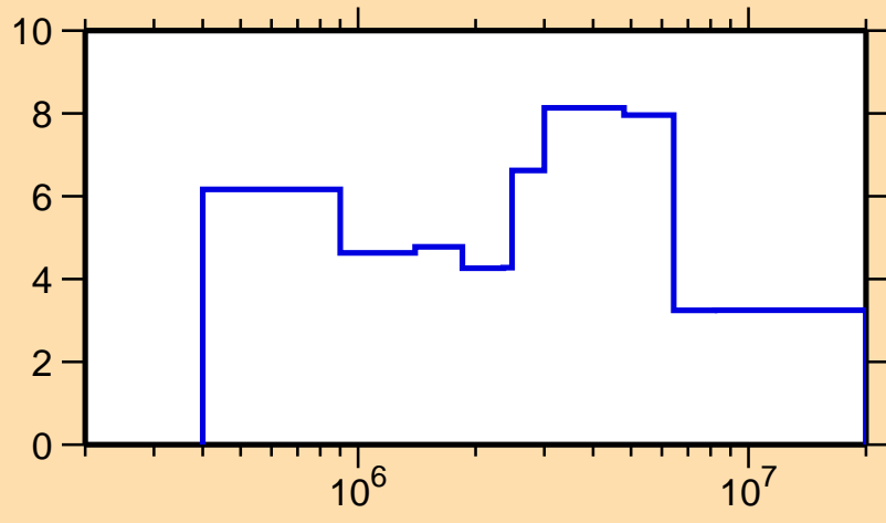
\Delta\sigma/\sigma vs. E for ^{157}\text{Er}(n, \text{el.})
