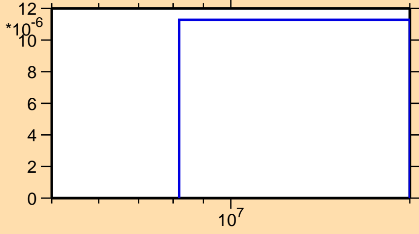
\sigma vs. E for ^{157}\text{Er}(n,2n\alpha)
