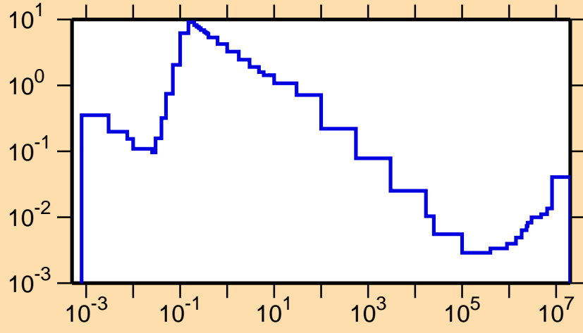
\sigma vs. E for ^{157}\text{Er}(n,p)
