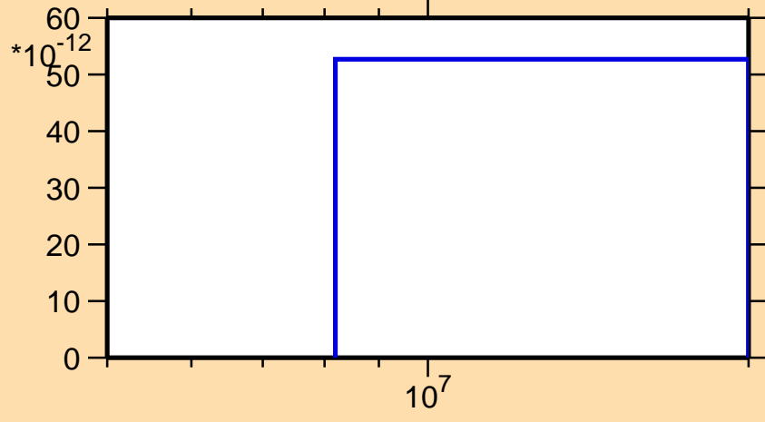
\sigma vs. E for ^{157}\text{Er}(\text{mt } 45)
