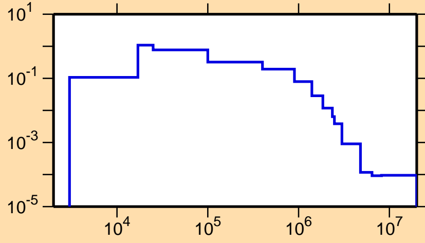
\sigma vs. E for ^{157}\text{Er}(n,n_1)
