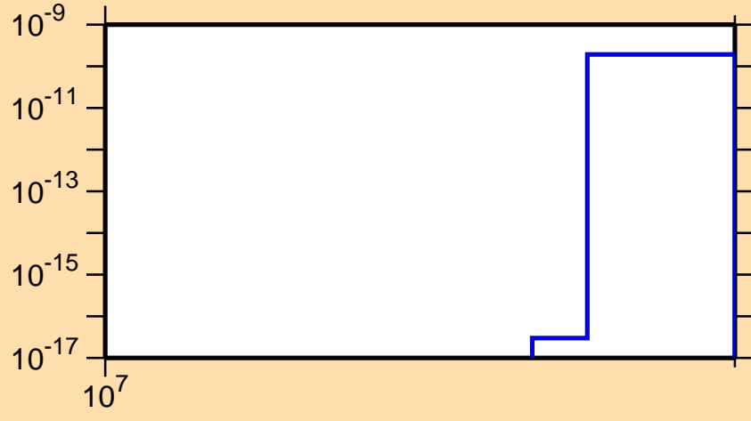
\sigma vs. E for ^{158}\text{Er}(n,nt)
