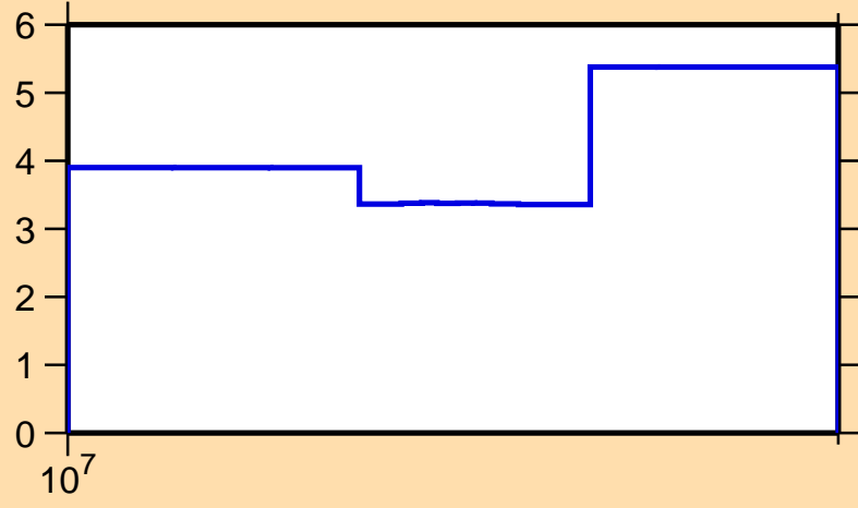
\Delta\sigma/\sigma vs. E for ^{158}\text{Er}(n,\text{el.})
