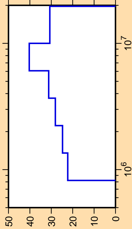
\Delta\sigma/\sigma vs. E for ^{158}\text{Er}(n,n_4)
