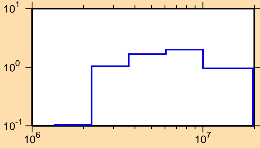
\sigma vs. E for ^{158}\text{Er}(n,n\text{cont.})
