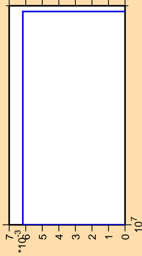
\Delta\sigma/\sigma vs. E for ^{158}\text{Er} (mt 34)
