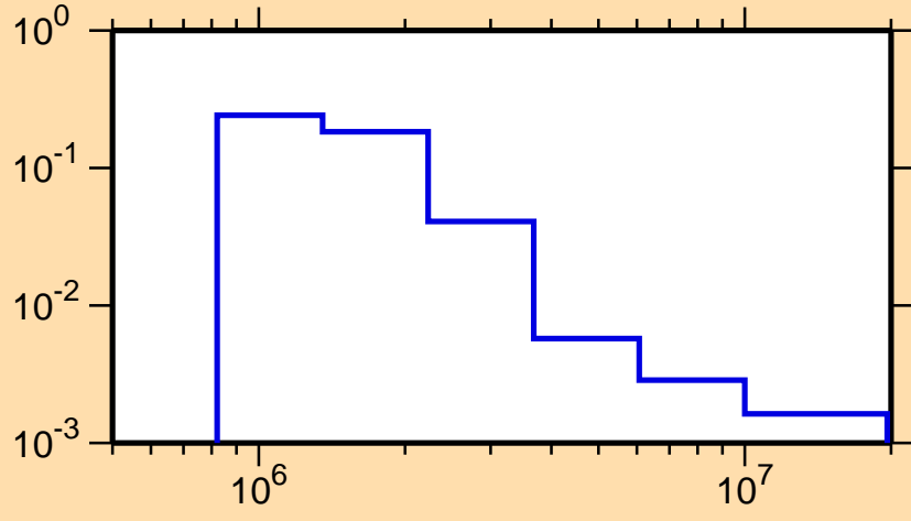
\sigma vs. E for ^{158}\text{Er}(n,n_4)
