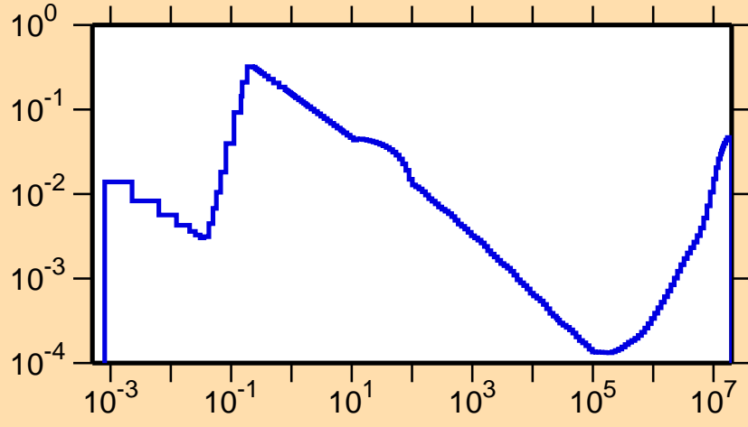
\sigma vs. E for ^{159}\text{Er}(n,p)
