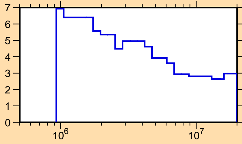
\Delta\sigma/\sigma vs. E for ^{159}\text{Er}(n,\text{nonel.})
