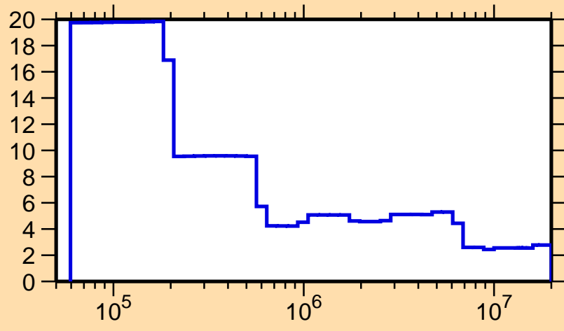
\Delta\sigma/\sigma vs. E for ^{159}\text{Er}(n,\text{el.})
