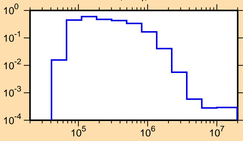
\sigma vs. E for ^{159}\text{Er}(n,n_1)
