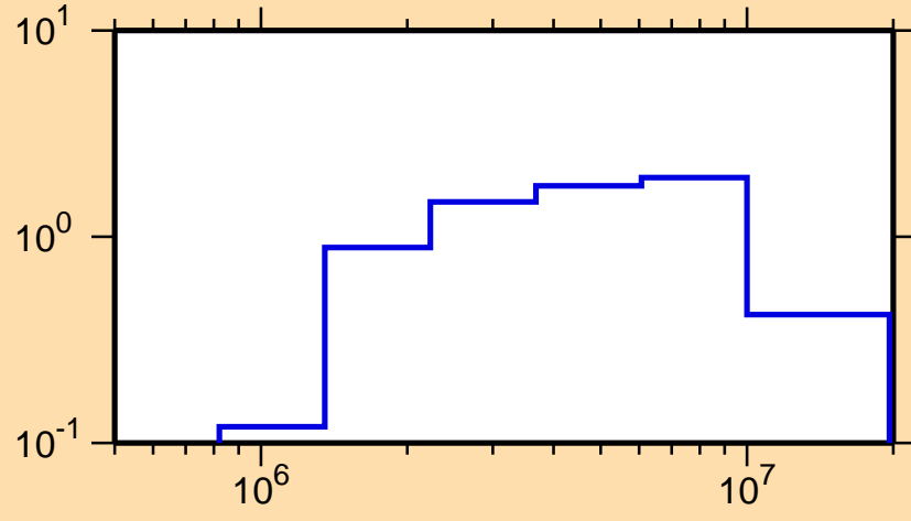
\sigma vs. E for ^{159}\text{Er}(n,n\text{cont.})
