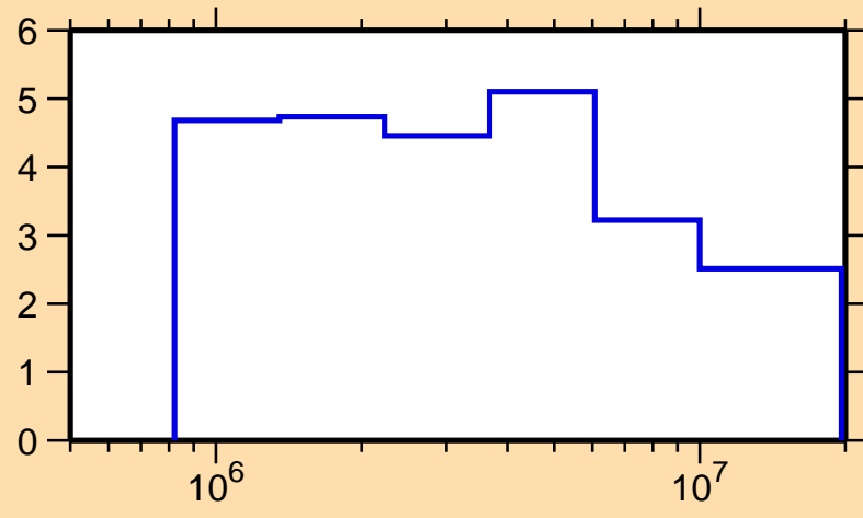
\Delta\sigma/\sigma vs. E for ^{159}\text{Er}(n,\text{el.})
