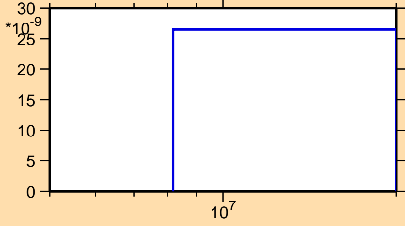
\sigma vs. E for ^{159}\text{Er}(n,\text{He3})
