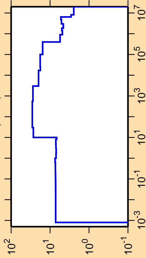
\Delta\sigma/\sigma vs. E for ^{159}\text{Er}(n,\text{el.})
