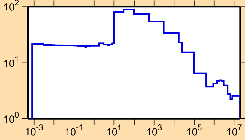
\sigma vs. E for ^{159}\text{Er}(n,\text{el.})
