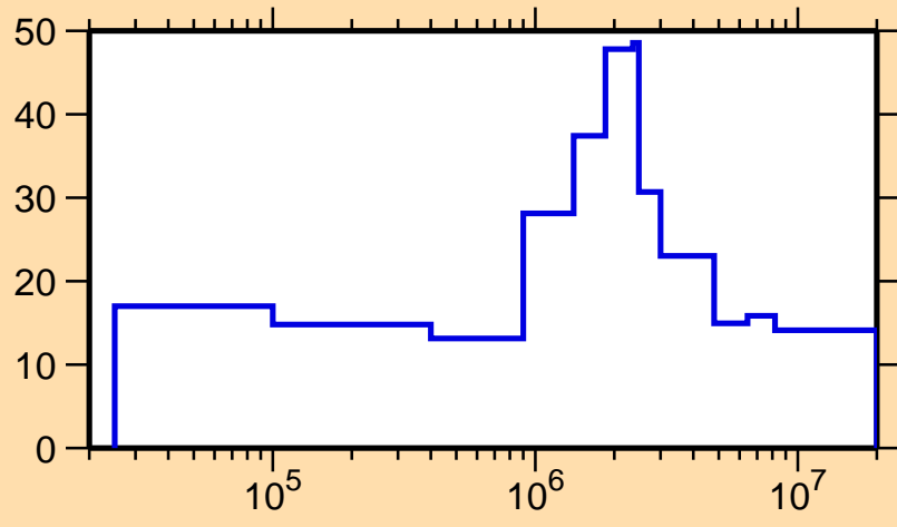
\Delta\sigma/\sigma vs. E for ^{159}\text{Er}(n,n_1)
