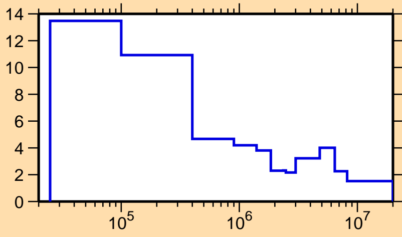
\Delta\sigma/\sigma vs. E for ^{159}\text{Er}(n,\text{tot.})
