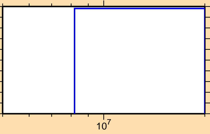
\sigma vs. E for ^{159}\text{Er}(\text{mt117})
