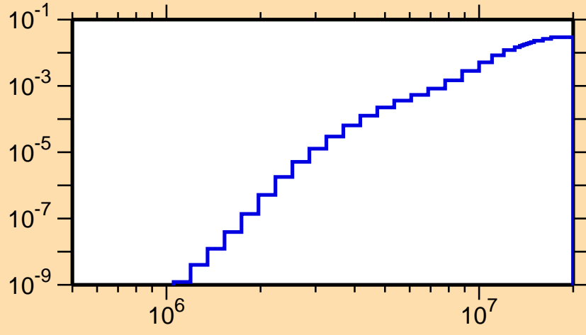
\sigma vs. E for ^{160}\text{Er}(n,p)
