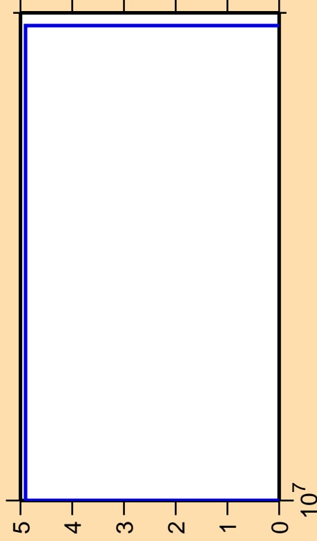
\Delta\sigma/\sigma vs. E for ^{160}\text{Er}(n,nt)
