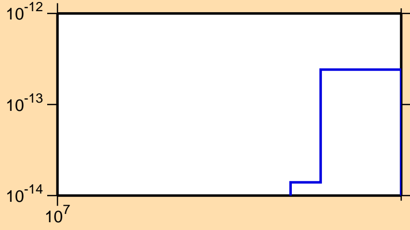
\sigma vs. E for ^{161}\text{Er}(\text{mt117})
