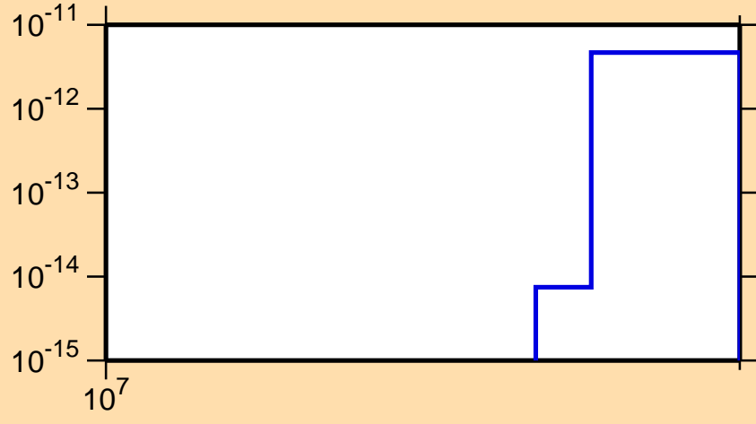
\sigma vs. E for ^{161}\text{Er} (mt 34)
