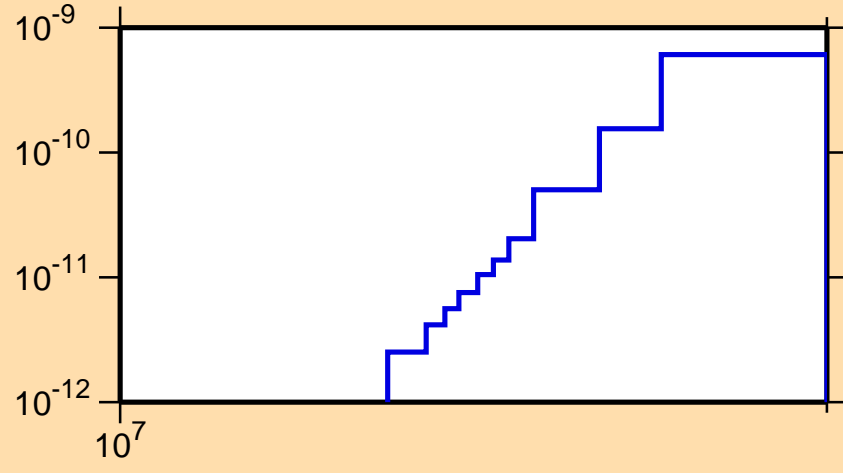
\sigma vs. E for ^{162}\text{Er}(n,p\alpha)
