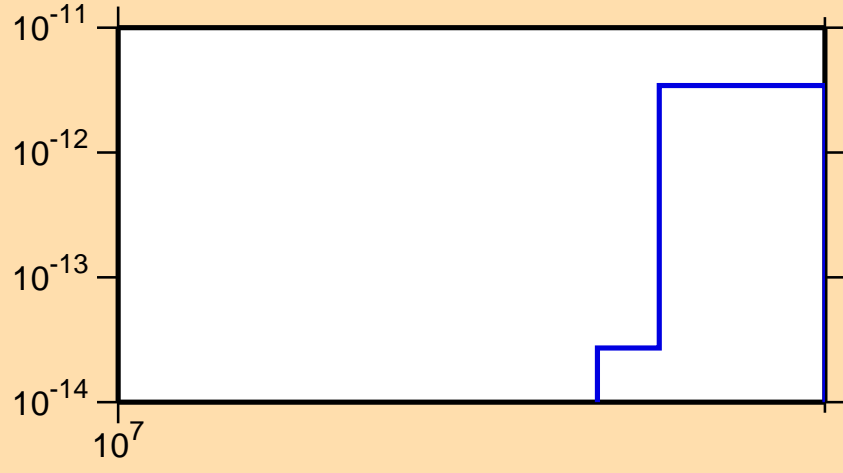
\sigma vs. E for ^{162}\text{Er}(n,\text{pd})
