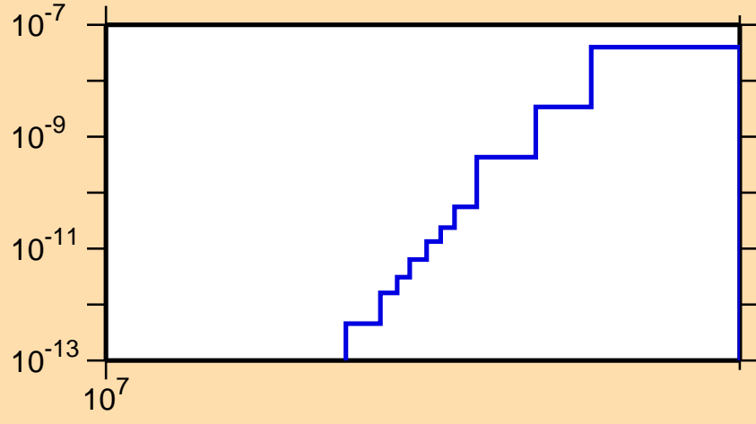
\sigma vs. E for ^{163}\text{Er}(n,\text{He3})
