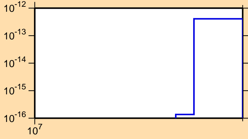
\sigma vs. E for ^{163}\text{Er} (mt 34)
